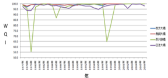
Fig.1 WQI in Yodo River
