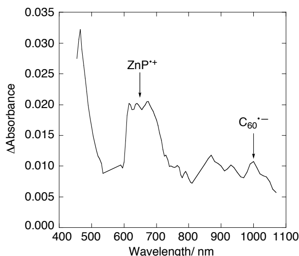
Figure 10. Transient absorption spectrum of \text{ZnP-ester}+\text{C}_{60}\text{-ester}/\text{SnO}_2/\text{ITO} at time delay of 10 ps excited at 555 nm.
