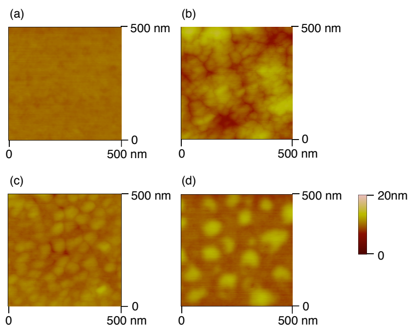
Figure 5. AFM images of (a) ZnP-acid, (b) ZnP-ester, (c) C_{60} -acid, and (d) C_{60} -ester on mica substrate. The color scale represents the height topography with bright and dark representing the highest and lowest features, respectively. An equimolar DMF solution of porphyrin (ZnP-acid, ZnP-ester) or fullerene ( C_{60} -acid, C_{60} -ester) was spin-coated onto freshly cleaved mica.
