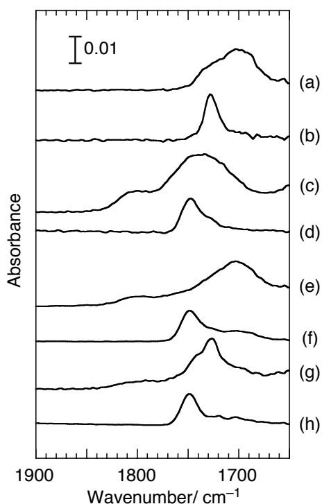
Figure 4. IRRA spectra in the C=O stretching region (1900–1650 \text{cm}^{-1} ) for the thin films of porphyrin and/or fullerene spin-coated on gold surface as (a) ZnP-acid, (b) ZnP-ester, (c) \text{C}_{60} -acid, (d) \text{C}_{60} -ester, (e) ZnP-acid+ \text{C}_{60} -acid, (f) ZnP-acid+ \text{C}_{60} -ester, (g) ZnP-ester+ \text{C}_{60} -acid and (h) ZnP-ester+ \text{C}_{60} -ester. An equimolar DMF solution of porphyrin (ZnP-acid, ZnP-ester) and/or fullerene ( \text{C}_{60} -acid, \text{C}_{60} -ester) was spin-coated onto gold surfaces.
