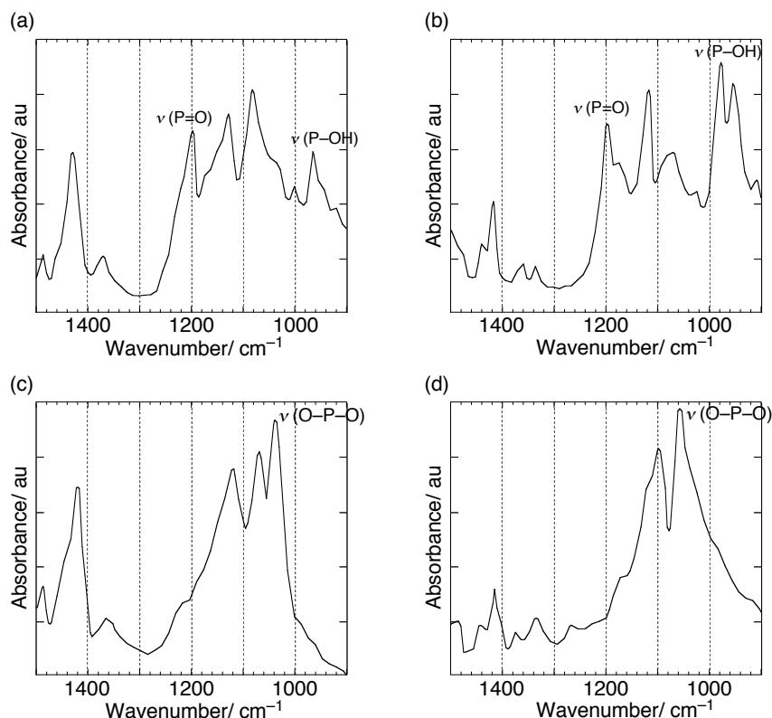
Figure 8. ATR-FTIR spectra of (a) TP and (b) PP , and (c) \text{TiO}_2/\text{TP} and (d) \text{TiO}_2/\text{PP} electrodes. The absorption arising from the corresponding bare \text{TiO}_2 electrode was subtracted from the spectra of \text{TiO}_2/\text{TP} and \text{TiO}_2/\text{PP} to obtain those of (c) and (d).
