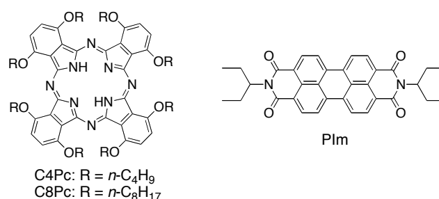
Figure 1. Phthalocyanine (C4Pc, C8Pc) and erylene diimide (PIm) used in this study.
