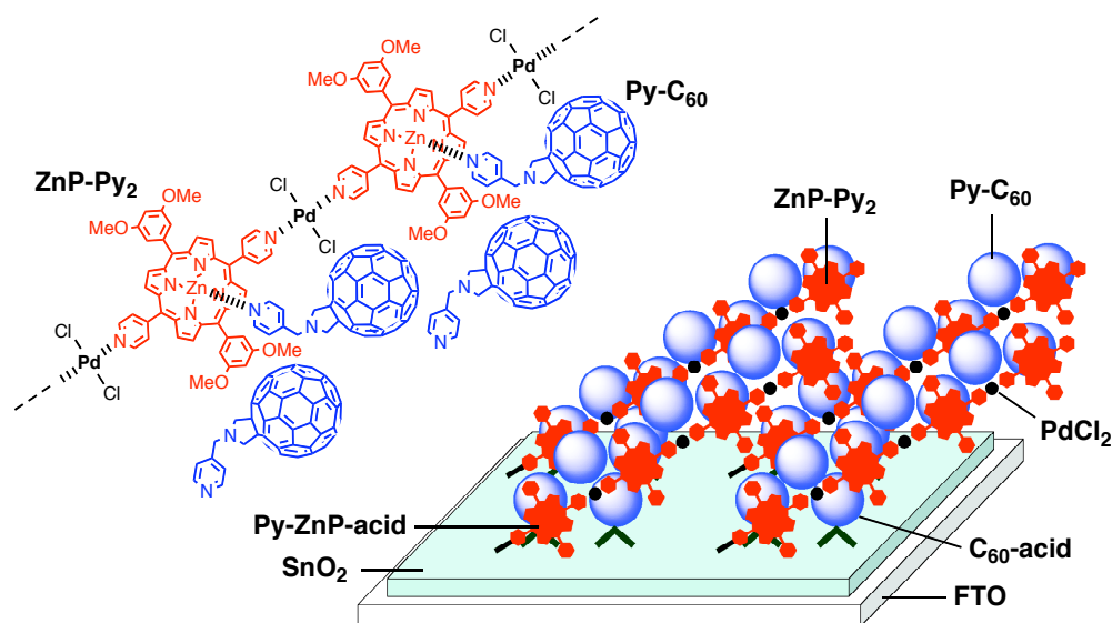
Figure 1. Schematic porphyrin-fullerene arrays on a \text{SnO}_2 electrode.
