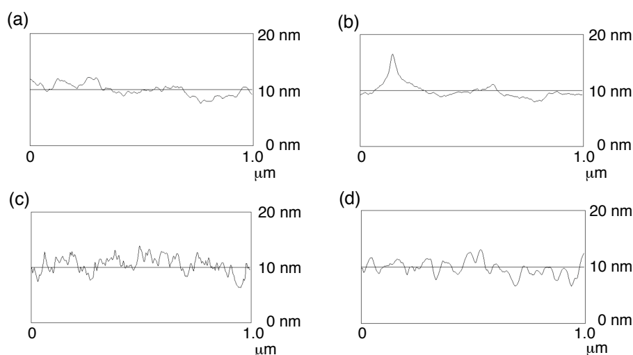
Figure 6. Section profiles of AFM images of (a) ZnP-acid+ C_{60} -acid/SnO 2 /ITO, (b) ZnP-ester+ C_{60} -acid/SnO 2 /ITO, (c) ZnP-acid+ C_{60} -ester/SnO 2 /ITO, and (d) ZnP-ester+ C_{60} -ester/SnO 2 /ITO ([ZnP]:[ C_{60} ] = 1:1) electrodes prepared by the spin-coating method.
