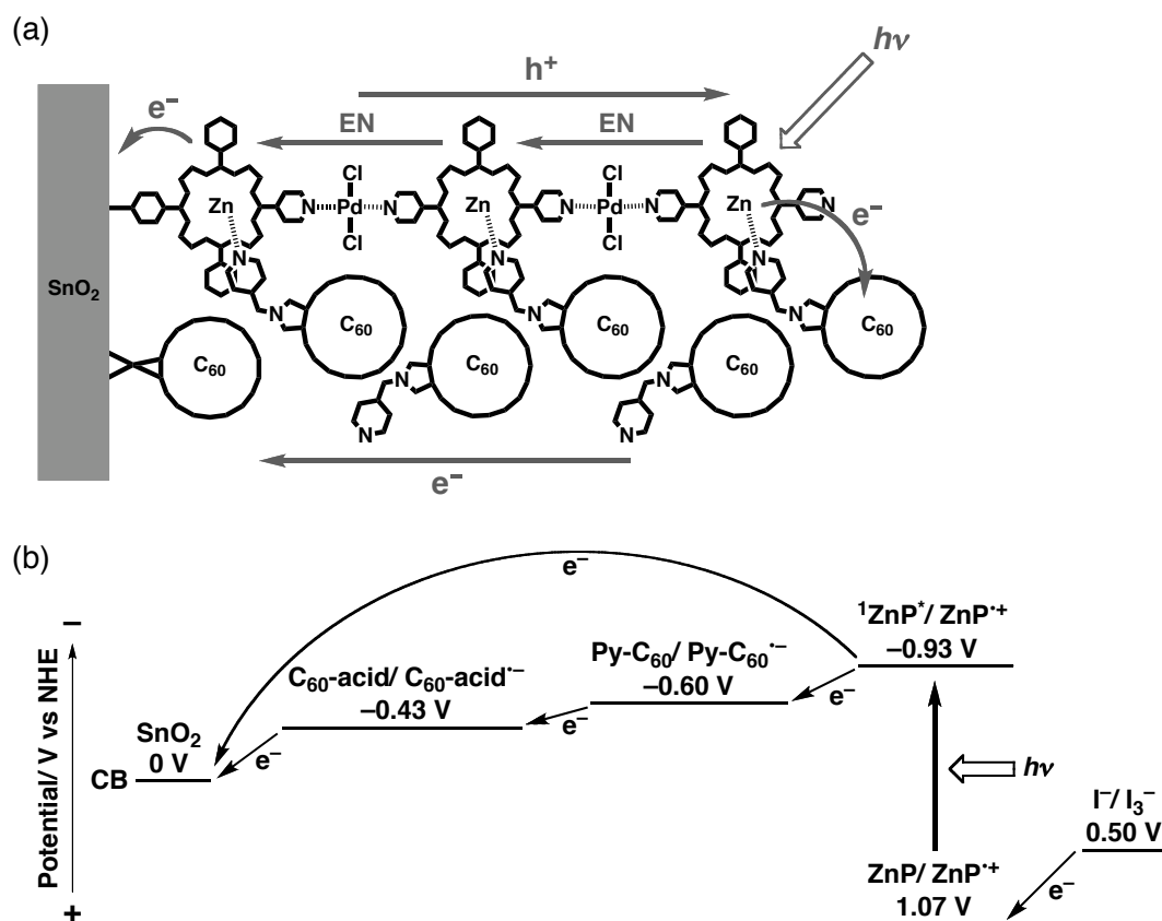
Scheme 4. (a) Schematic illustration for the photocurrent generation in the \text{SnO}_2/\text{C}_{60}\text{-acid}+(\text{ZnP})_n+\text{Py-C}_{60} systems and (b) its energy diagram. The levels of \text{C}_{60}\text{-acid} and \text{Py-C}_{60} were determined electrochemically from the first reduction potentials of \text{C}_{60}\text{-acid} and \text{Py-C}_{60} in chloroform.
