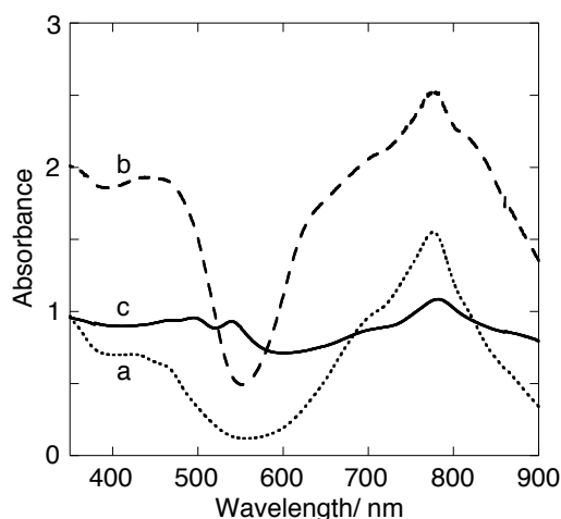
Figure 6. The absorption spectra of ITO/SnO 2 /(C8Pc) m , prepared from the cluster solution ((a) 0.25 mM, dotted line; (b) 0.50 mM, dashed line), and of ITO/SnO 2 /(C8Pc+PIm) m , prepared from the cluster solution ((c) [C8Pc] = [PIm] = 0.50 mM, solid line).
