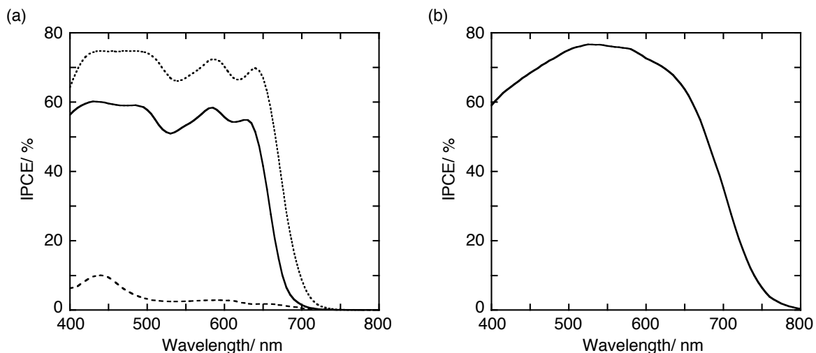
Figure 11. Photocurrent action spectra of TiO 2 /ZnBQA+CDCA (solid line), TiO 2 /ZnQCA+CDCA (dashed line), TiO 2 /ZnQMA+CDCA (dotted line), and (b) N719-sensitized cell.
