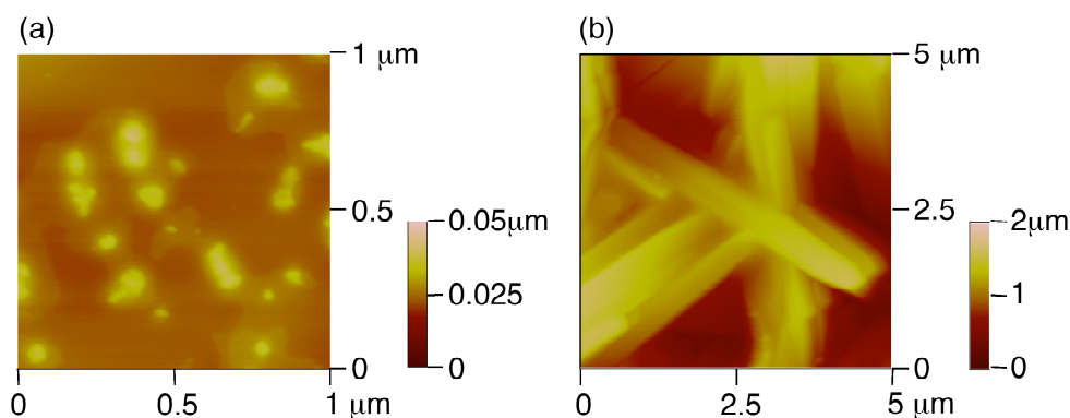
Figure 7. Tapping mode atomic force micrograph of (a) ITO/SnO 2 /(C8Pc) m and (b) ITO/SnO 2 /(C8Pc+PIm) m electrodes in air. The samples were prepared from the cluster solutions ((a) [C8Pc] = 0.50 mM) and ((b) [C8Pc] = [PIm] = 0.50 mM), respectively.
