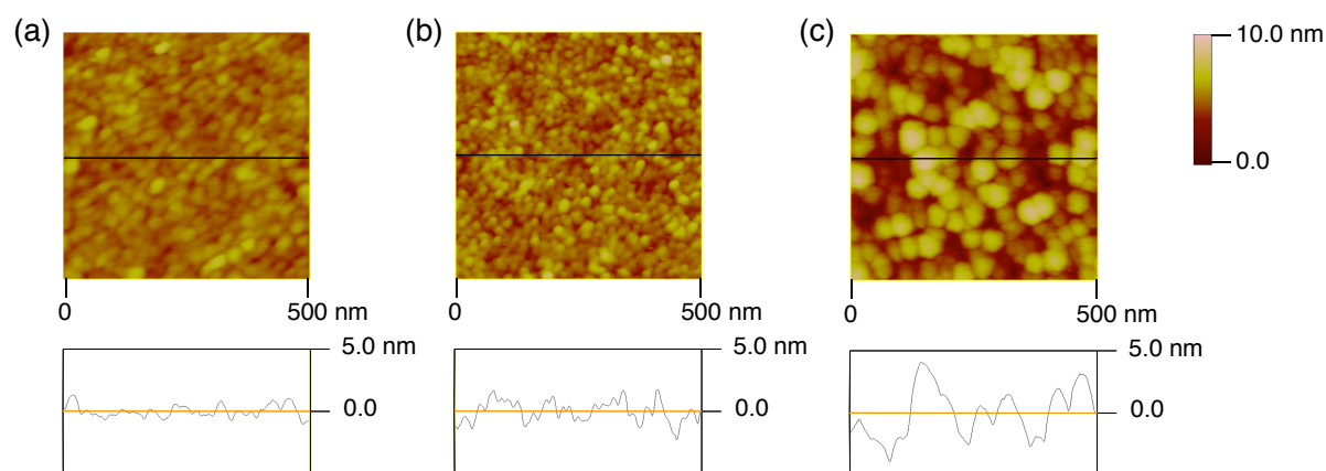
Figure 10. AFM images for surface morphology of (a) \text{SnO}_2/(\text{ZnP})_2 , (b) \text{SnO}_2/(\text{ZnP})_4 , (c) \text{SnO}_2/(\text{ZnP})_6 . The \text{SnO}_2 film was prepared on a glass substrate.
