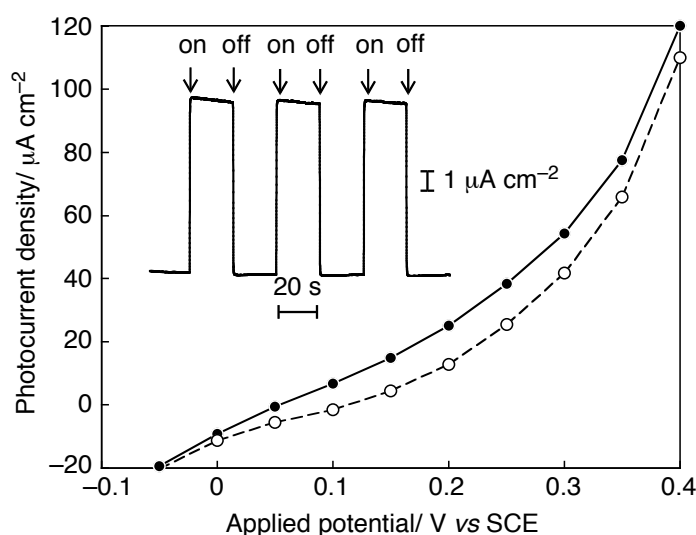
Figure 7. Photocurrent vs applied potential curves of \text{ZnP-acid+C}_{60}\text{-acid}/\text{SnO}_2/\text{ITO} system. The dark currents are shown as dashed line with open circles. Experimental conditions were as follows; excitation power: 85 \mu\text{W cm}^{-2} ( \lambda_{\text{ex}} = 435 nm); absorbance: 1.00 at excitation wavelength; thickness of \text{SnO}_2 layer: 1.1 \mu\text{m} ; 0.5 M LiI and 0.01 M \text{I}_2 in acetonitrile. The photoelectrochemical response at applied potential of 0.15 V vs SCE is shown as an inset.
