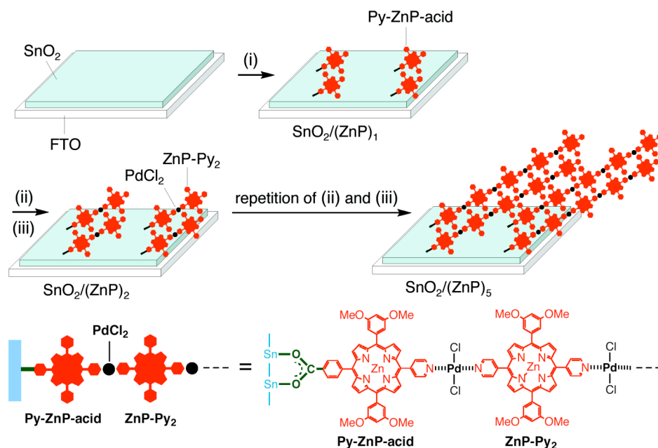
Scheme 1. Procedures for preparation of porphyrin arrays on a \text{SnO}_2 electrode. (i) A \text{SnO}_2 electrode was immersed into Py-ZnP-acid (0.2 mM in DMF) for 4 h, and then washed with DMF. (ii) The \text{SnO}_2 electrode modified with the porphyrins was immersed into \text{K}_2\text{PdCl}_4 (3.0 mM in water) for 20 min, and then washed with water and finally immersed into MeOH for 20 min. (iii) The \text{SnO}_2 electrode was immersed into ZnP-Py 2 (0.2 mM in \text{CHCl}_3/\text{MeOH} (3:1, v/v)) for 20 min, and then washed with \text{CHCl}_3 , and finally immersed into MeOH for 20 min to yield \text{SnO}_2/(\text{ZnP})_n ( n = 1-8 ) electrode.
