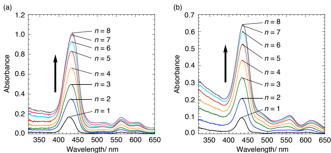
Figure 3. Spectral change in the absorption spectra of electrodes after successive assembly of ZnP-Py 2 on the electrode modified with (a) Py-ZnP-acid ( \text{SnO}_2/(\text{ZnP})_n ) and (b) Py-ZnP-acid and \text{C}_{60} -acid ( \text{SnO}_2/\text{C}_{60}\text{-acid}+(\text{ZnP})_n ). The absorbance arising from the \text{SnO}_2 electrode was subtracted from the spectrum.
