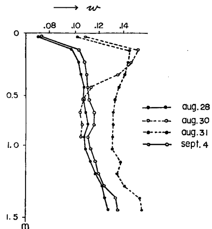
Fig. 8 Graphic curves of hydrous ratio through the neutron hydrogic mater.
