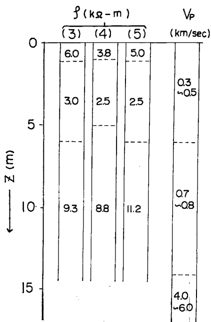
Fig. 9 Resulting logs of resistivity and seismic prospecting.
