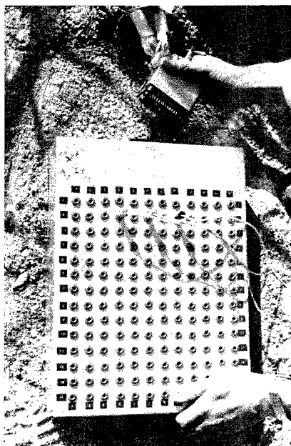
Photo. 2 Terminal-box for multi-electrodes method.
