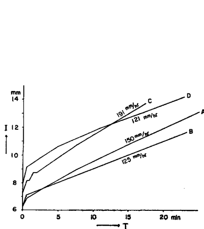
Fig. 7 Curves of infiltration rate. I ; infiltration capacity
