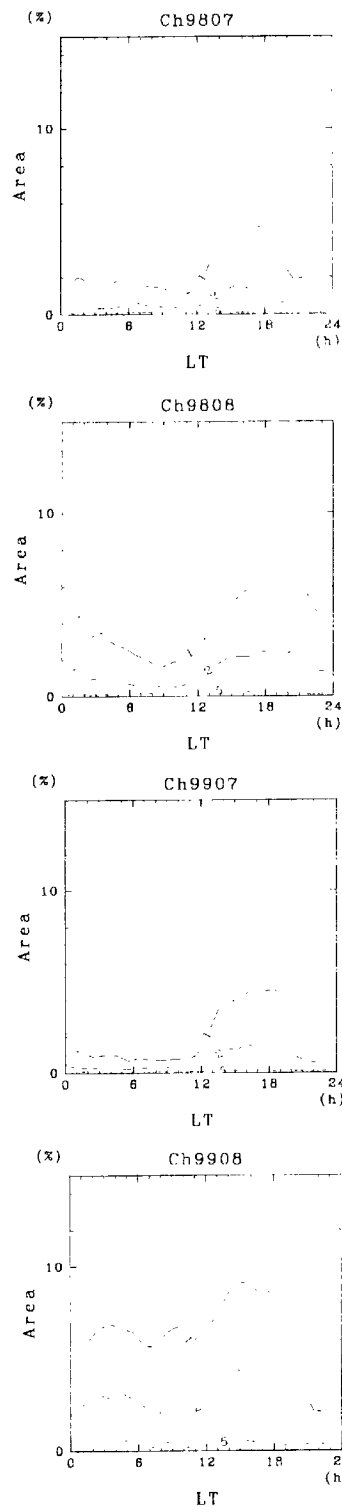
Fig. 10. Monthly averaged diurnal variation of echo area (%) in the lowest elevation angle at Chiang Mai in (top) July 1998, (second) August 1998, (third) July 1999, and (bottom) August 1999. Solid, dashed and dotted lines indicate 1, 2 and 5 dBZ, respectively.
