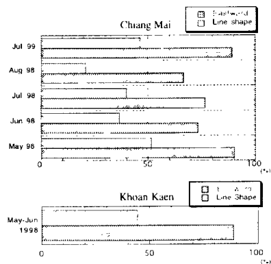
Fig. 8. Ratio (%) of days when eastward moving echoes and line-shaped echoes are observed at (upper panel) Chiang Mai and (lower panel) Khoan Kaen.
