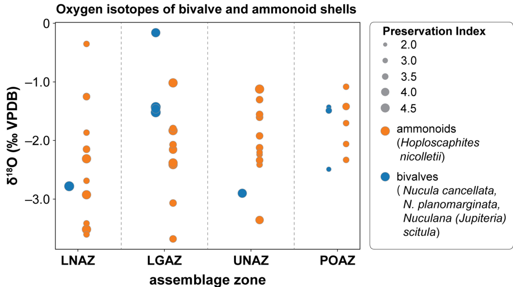
Fig. 8 Results of \delta^{18}\text{O}_{\text{shell}} analysis. The size of the markers represents the preservation index (Knoll et al., 2016). Orange markers = ammonoids ( Hoploscaphites nicolletii ) from Witts et al. (2020). Blue markers = bivalves [ Nucula cancellata , N. planomarginata , Nuculana ( Jupiteria ) scitula ]
