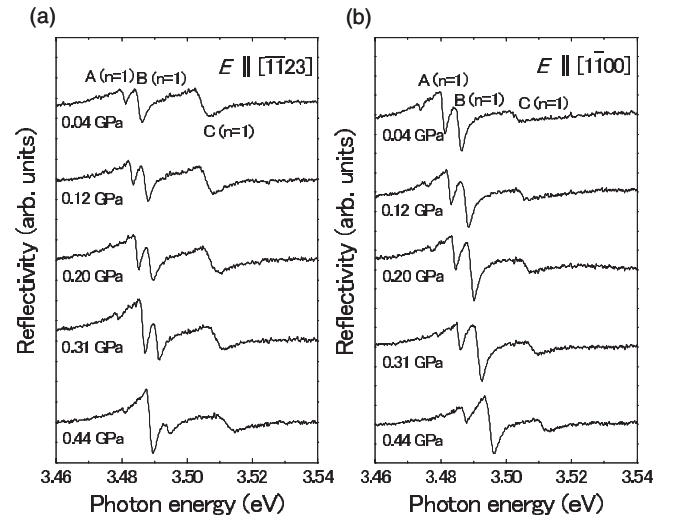
FIG. 9. Reflectance spectra of the (11 \bar{2} 2) plane GaN bulk substrate under uniaxial stress P \parallel [\bar{1}\bar{1}23] . (a) E \parallel [\bar{1}\bar{1}23] and (b) E \parallel [1\bar{1}00] .
