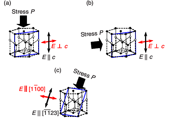
FIG. 4. (Color online) Experimental configurations (a) P \parallel c , (b) P \perp c , and (c) P \parallel [\bar{1}\bar{1}\bar{2}3] .
