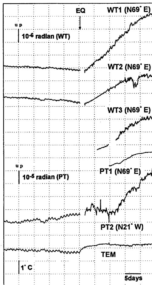
Fig. 6. Tilt data (hourly value) observed by water-tube tiltmeters and pendulum tiltmeters during 50 days before and after the earthquake.
