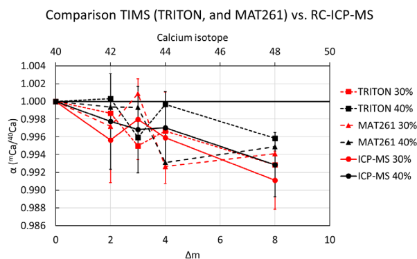
Fig 3. The calculated separation factor ( \alpha ) per mass unit of the ICP-MS (Agilent 7900) and TIMS (TRITON and MAT261)
