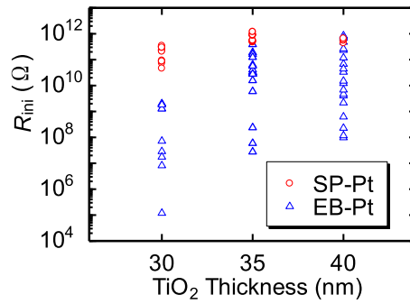
FIG. 6. TiO 2 thickness dependence of initial resistance at 1 V ( R_{\text{ini}} ) in the SP-Pt and EB-Pt samples.
