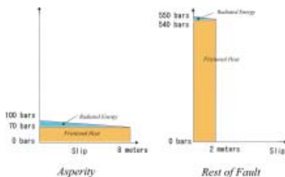
Fig. 8. Energy budgets for the northern (asperity) and southern portions of the fault.
