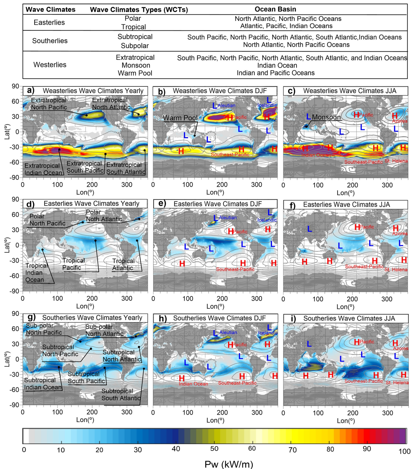
Figure 1. Global wave climates classified by dynamic clustering. P_w ( \text{kW/m} ), yearly averaged (a, d, g), DJF (b, e, h), and JJA (c, f, i), of the westerlies (a, b, c), easterlies (d, e, f), and southerlies (g, h, i) wave climates. Gray contour lines indicate the average sea level pressure (SLP). H and L indicate the high and low-pressure centers of the SLP.
