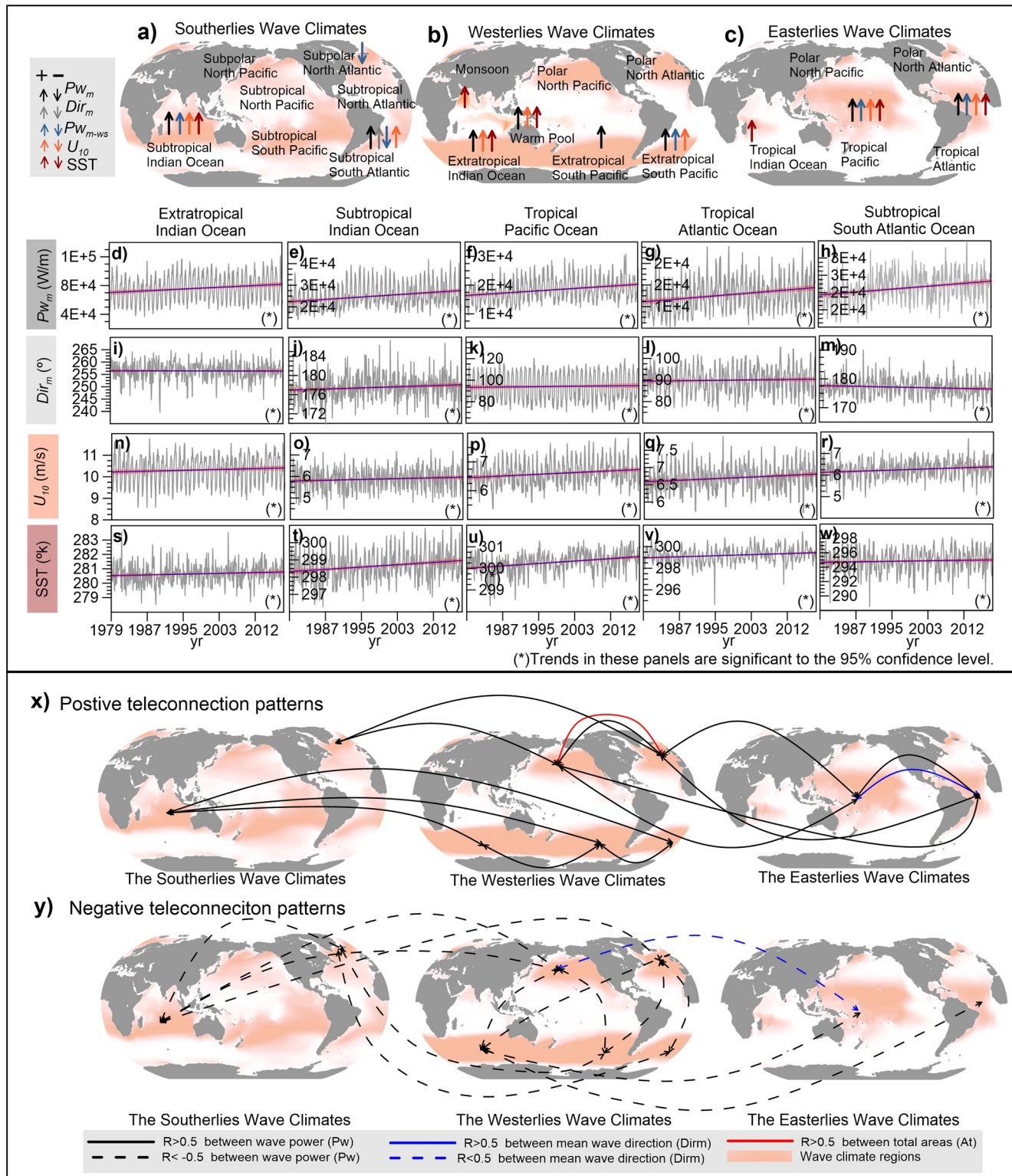
Figure 3. Trends of wave power ( Pw_m ), mean wave direction ( Dir_m ), wind-sea wave power ( Pw_{m-ws} ), wind velocity U_{10} , and sea surface temperature (SST) for (a) southerlies, (b) westerlies, and (c) easterlies wave climate types (WCTs). Time series and trends of WCTs (d)–(h) Pw_m (i–m) Dir_m (n–r) U_{10} , and (s–w) SST, for (d, i, n, s) the extratropical Indian Ocean (e, j, o, t) subtropical Indian Ocean (f, k, p, u) tropical Pacific (g, l, q, v) tropical Atlantic, and (h, m, r, w) subtropical South Atlantic. Correlation coefficients R for mean wave power, mean wave direction, and total area between the WCTs, x) positive correlation denoting either an increase/increase or decrease/decrease global teleconnection pattern, and y) negative correlation indicating an inverse (i.e., increase/decrease) teleconnection pattern.
