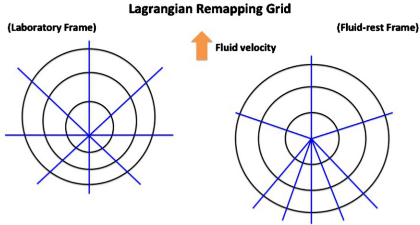
Figure 4. Lagrangian remapped grid in the laboratory frame (left panel) and the Lorentz-transformed grid in the fluid restframe (right panel). The energy grid is isotropic in the fluid restframe whereas it becomes anisotropic in the laboratory frame. The angular grid, on the other hand, is uniform in the laboratory frame. (A color version of this figure is available in the online journal.)
