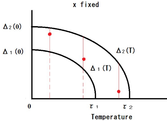
Figure 2: For each T , the solution u_0(T, x) lies between \Delta_1(T) and \Delta_2(T) .
