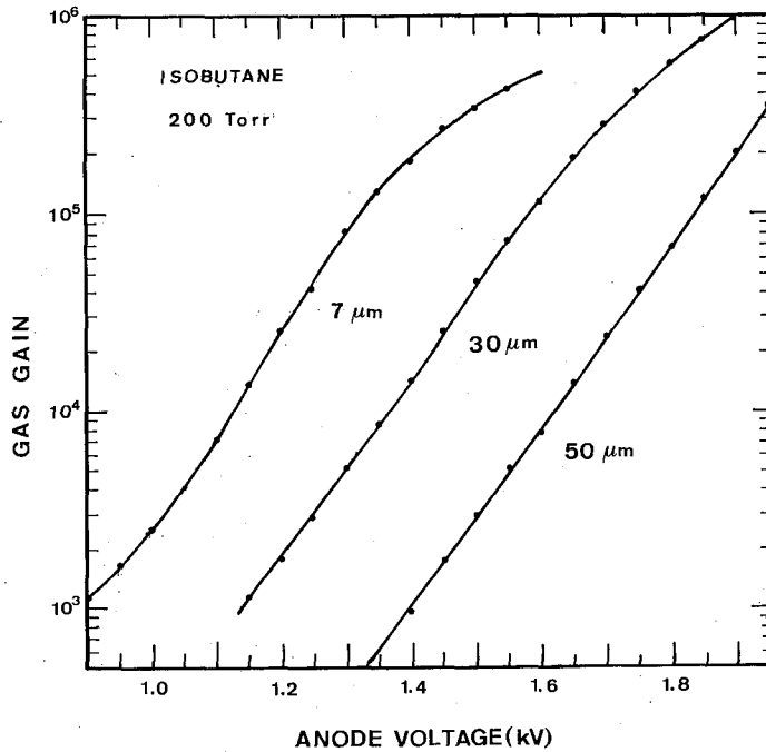
Fig. 1. Gas gains of the PSPC with wire anodes of various diameters, i.e., 7 , 30 and 50\text{ }\mu\text{m} . Values for gas gains have been estimated with the preamplifier output for 7.2\text{-keV} K conversion electrons from ^{57}\text{Co} . The counter gas is isobutane with a pressure of 200\text{ Torr} .
