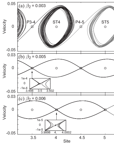
FIG. 9. Schematic relationship between coexisting ILMs and unstable manifolds for (a) \beta_2=0.003 , (b) 0.005, and (c) 0.006. The structure of the vicinity of an unstable ILM is shown in the insets. Unstable manifolds are located very close to the unstable ILM. There is no homo- or heteroclinic connection.
