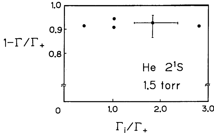
Fig. 6. Experimental plot of Eq. (8). The intercept gives the reflection coefficient R_e , and the slope gives the conversion coefficient c .
