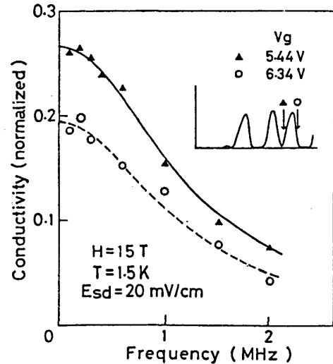
Fig. 4. The conductivity of the tail parts of the (0\pm-) peak relative to the peak value as a function of frequency. The solid and the broken curves represent the Drude-type frequency dependence for sample SN9.
