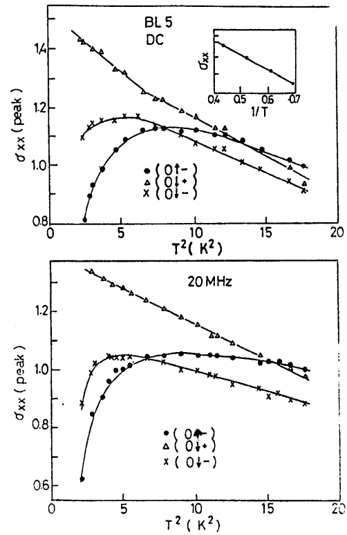
Fig. 6. Plot of (\sigma_{xx})_{\text{peak}} against T^2 for sample BL5. The inset shows the (\sigma_{xx})_{\text{peak}} vs. 1/T at the low temperature region.
