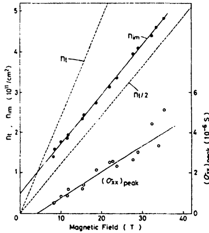
Fig. 2. (\sigma_{xx})_{peak} for (0\pm+) level, n_{im} and n_t as a function of magnetic field.
