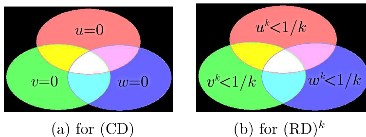
Figure 3. Colors for approximated regions which correspond to \Omega_1(t) (salmon), \Omega_2(t) (yellow green) and \Omega_3(t) (royal blue) respectively. (For interpretation of the references to color in this figure legend, the reader is referred to the web version of this article.)
