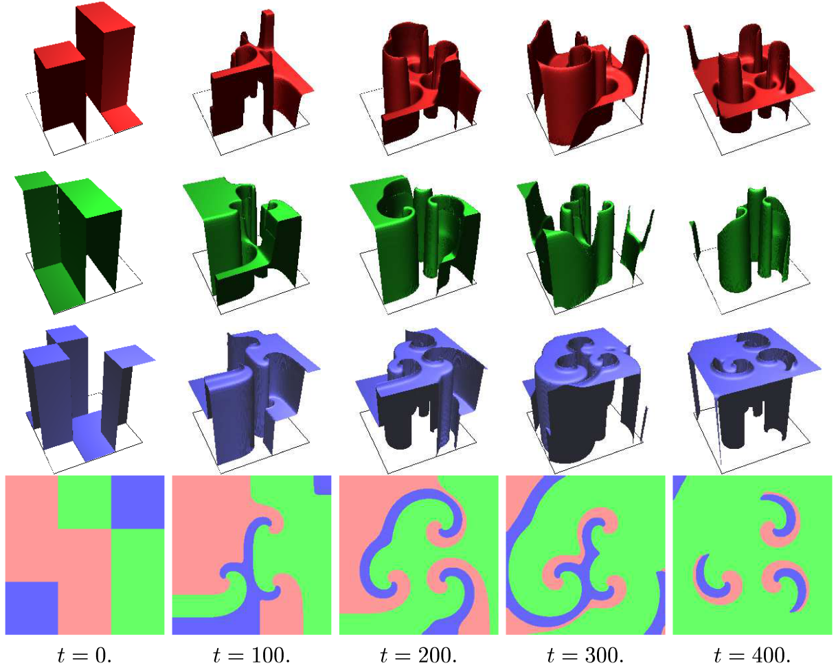
Figure 2. Numerical solutions of (CD).
