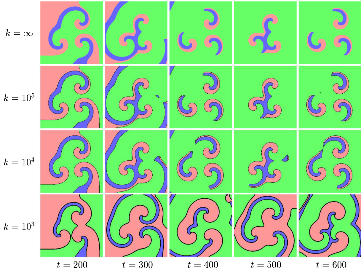
Figure 4. Numerical solutions for various choices of the parameter k . k = \infty implies the limit problem (CD).
