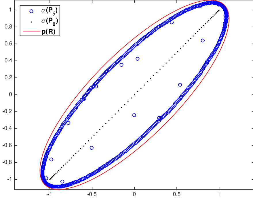
Figure 1: The black dots along the focal segment show the spectrum (obtained using MATLAB) of the unperturbed operator P with dimension N = 501 , a = 0.5 , b = i and \delta = 10^{-12} . The blue circles show the spectrum of the perturbed operator (1.6), and the red ellipse is the image of the symbol p .
