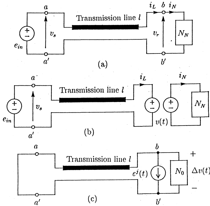
Fig. 1(a) A transmission line terminated by a nonlinear subnetwork (b) Partition the circuit into linear and nonlinear subnetwork using a substitution source v(t) (c) Sensitivity circuit for getting the variational value \Delta v(t)
