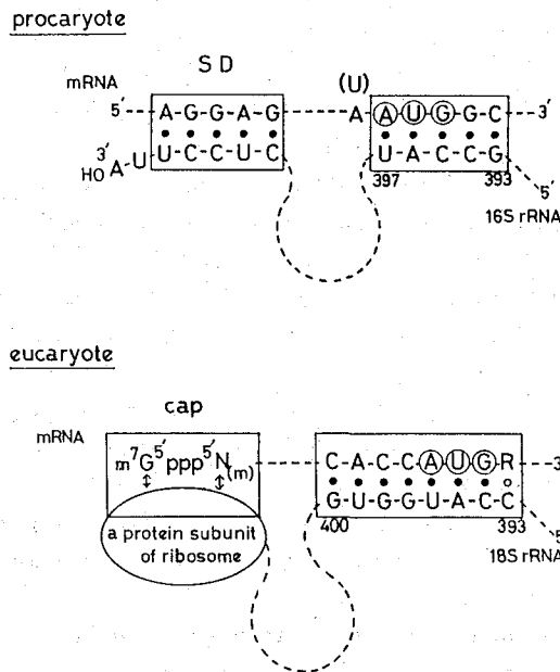
Fig. 4. Possible two binding sites are depicted schematically both for prokaryote and eukaryote. The cap site interacts probably with a protein subunit of ribosome shown by an ellipsoidal solid line. Dashed lines represent rRNAs.
