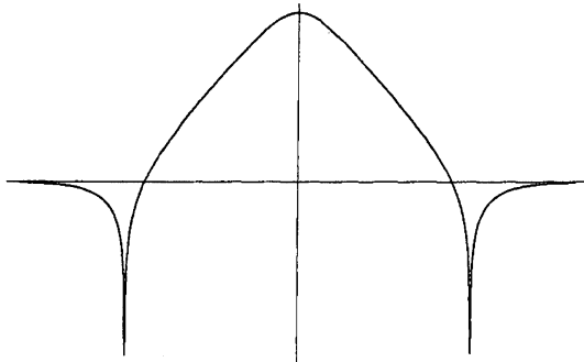
図 5 effective potential for v = 0.12, \theta_{12} = \pi
