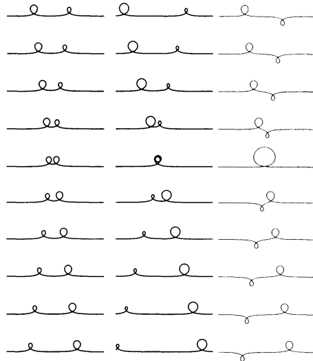
図 1 v = 0.12, v = 0.24, v = 0.12
