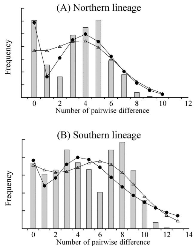
Fig. 5. Mismatch distributions of pairwise sequence differences between individuals from pooled data for each main lineage (A, northern lineage; B, southern lineage). The observed data (bars) were fitted to models of sudden population expansion (open triangles) or spatial expansion (closed circles).
