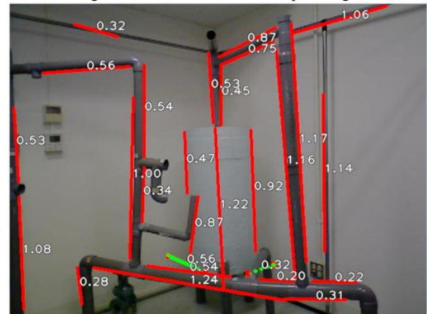
Fig. 6 An RGB image with all extracted line segments superimposed simultaneously.
