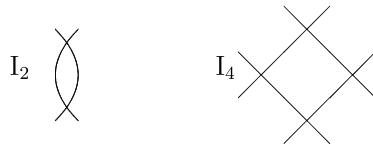
Figure 1: Singular fibres of types I_2 and I_4
