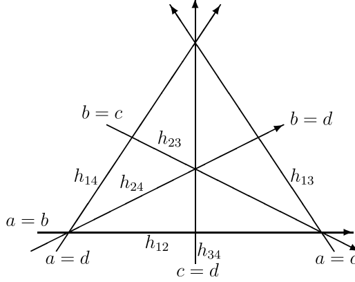
Figure 2: Singular locus D
