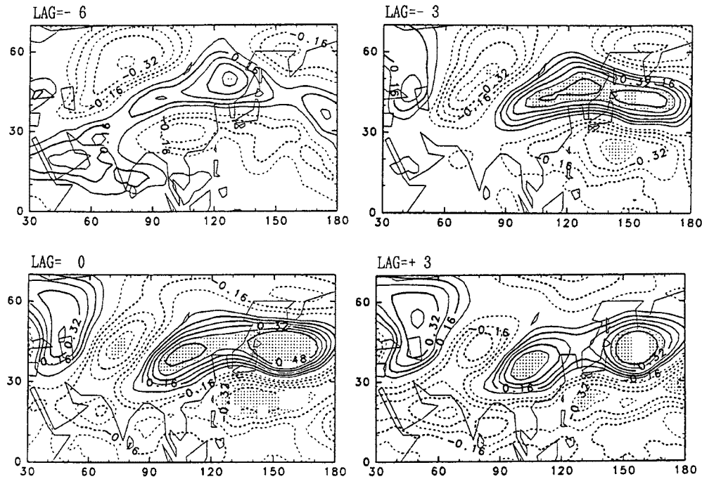
Fig. 7. Same as Fig. 6, except for EOF-2.
