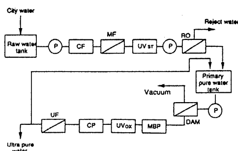
図 3.12: 超純水製造装置の概念図。CF:carbon filter, MF:membrane filter, UV st :ultraviolet sterilizer, RO:reverse osmosis membrane, DAM:membrane degasifier, MBP:mixed bed ion exchanger, UV ox :ultraviolet oxidizer, CP:cartridge polisher(small-sized mixed bed ion exchanger), UF:ultrafilter [17]
