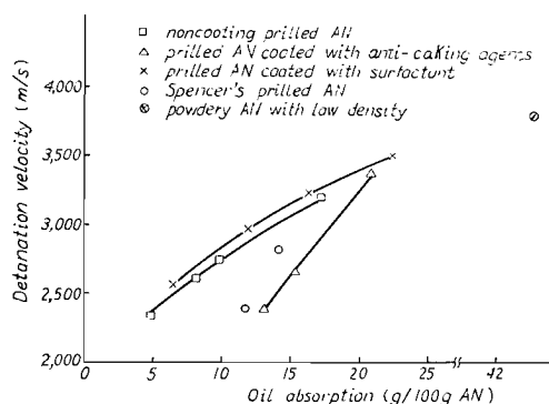
Fig. 4. Relation between oil absorption and detonation velocity.
