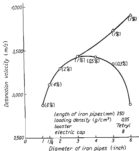
Fig. 10. Influence of weight of booster on detonation velocity. Ratio of booster per loaded ANFO is shown in parentheses.
