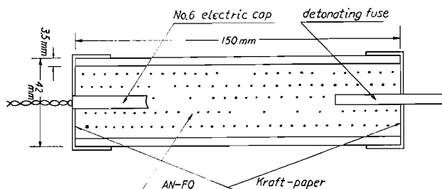
Fig. 8. Cap sensitivity test with vinyl chloride pipes.
