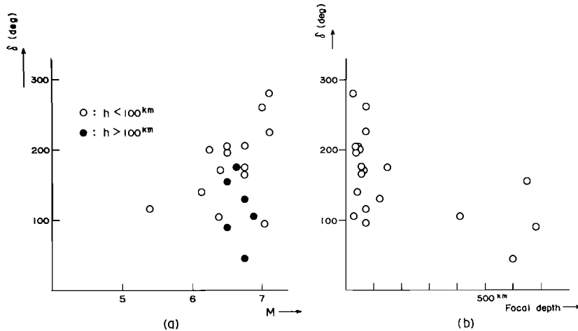
Fig. 47 (a) Relation between the magnitude ( M ) and the inclination of the phase spectrum ( \delta ).
