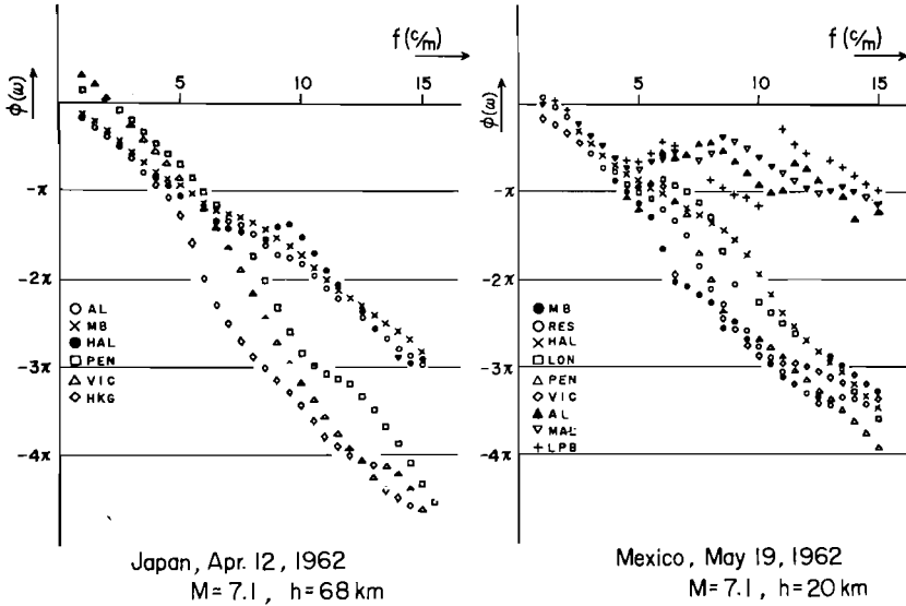
Fig. 41 Phase spectrum
