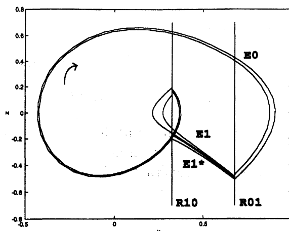
Figure 1: The slow flow for (4) with \theta = -0.25 . The very thin strips \mathcal{R}_{1 \rightarrow 0} and \mathcal{R}_{0 \rightarrow 1} indicate the domains where the fast flow possibly has a connecting orbit.
