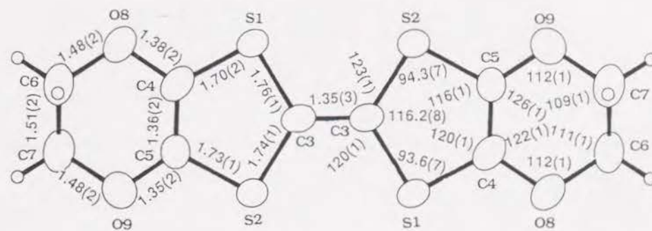
Figure A5. Bond lengths (Å) and angles (deg) in (BEDO-TTF) 10 (CF) 4 (H 2 O) 3 (33)
