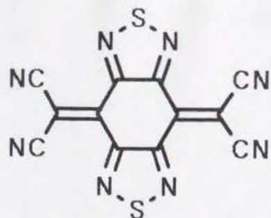
BTDA-TCNQ
