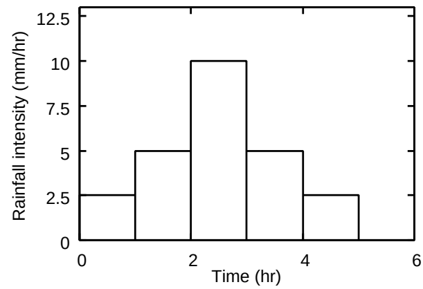
Figure 16. Rainfall intensity for Test 4.
