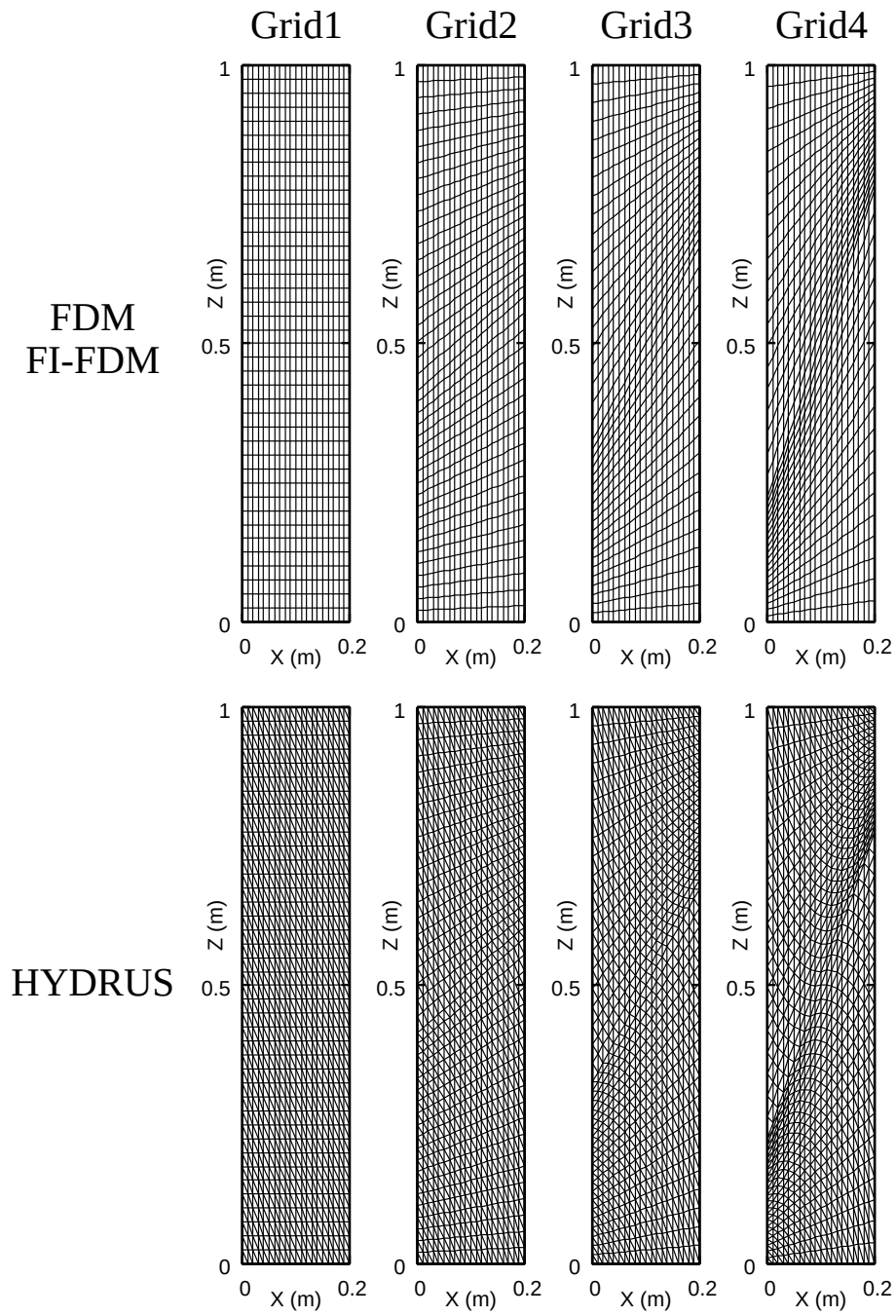
Figure 7. Four types of grids used in Test 2 ( 20 \times 40 ).
