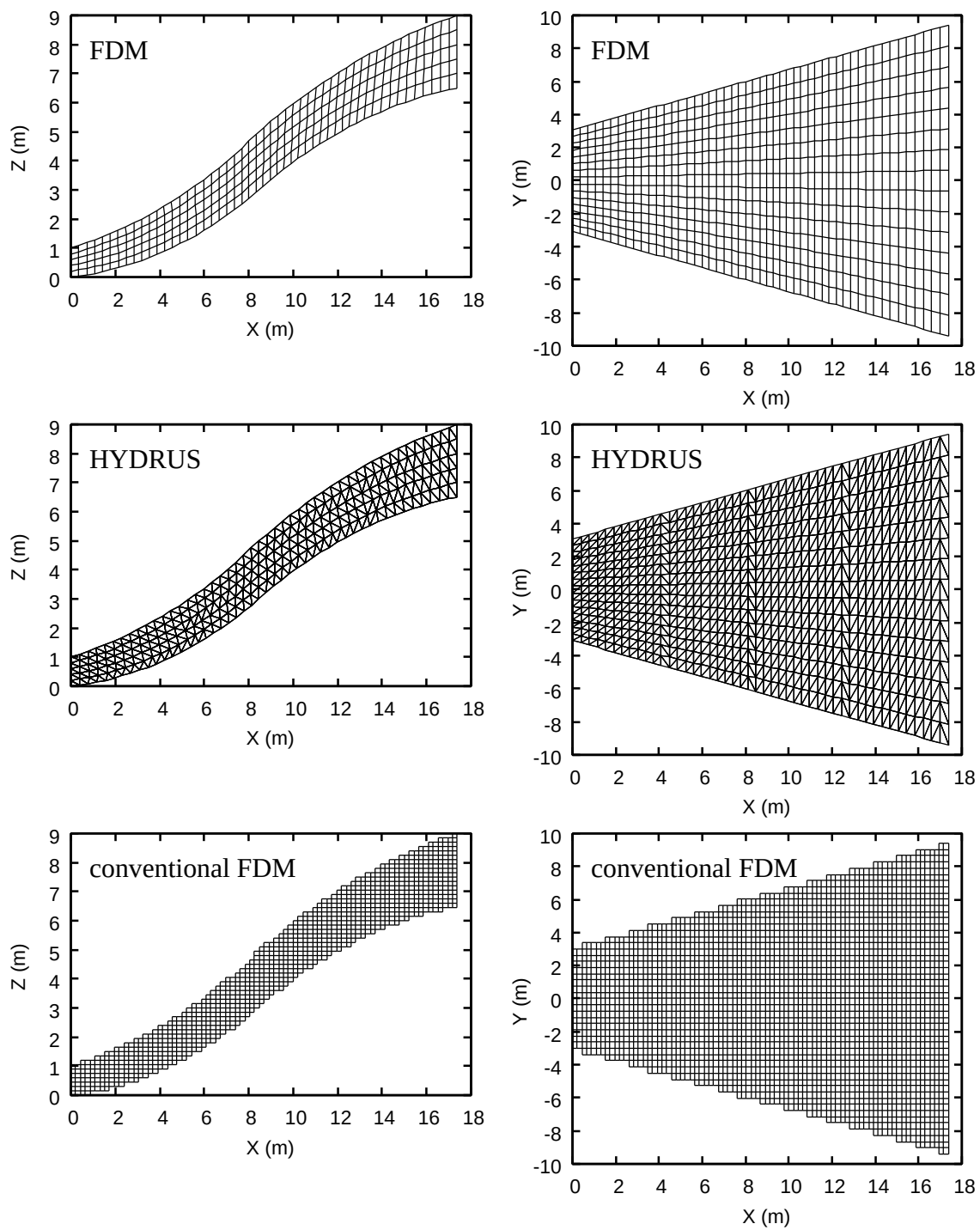
Figure 15. Grids used in Test 4; left side describes vertical sections from x,y coordinate (9,-10) and right side gives plan views.
