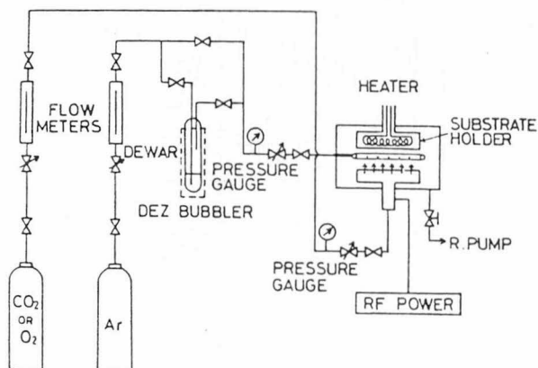
Fig.5.3. Schematic diagram of the PE-MO-CVD system.
