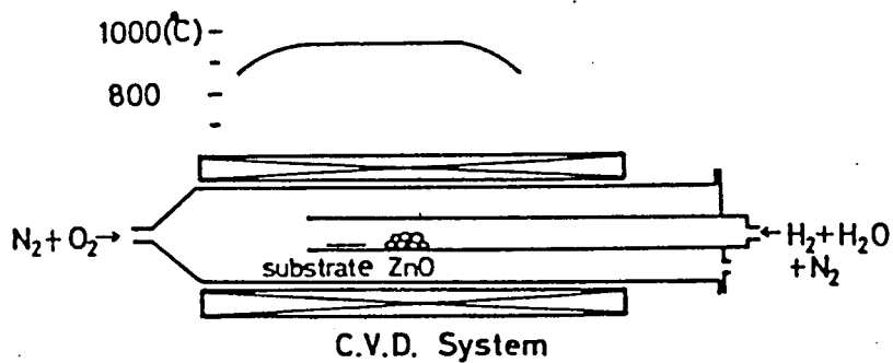
Fig.2.4. Schematic diagram of the CVD system.
