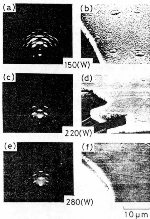
Fig.5.10. RHEED patterns and SEM micrographs of films prepared at different rf input powers: (a) and (b) 150W, (c) and (d) 220W, and (e) and (f) 280W.
