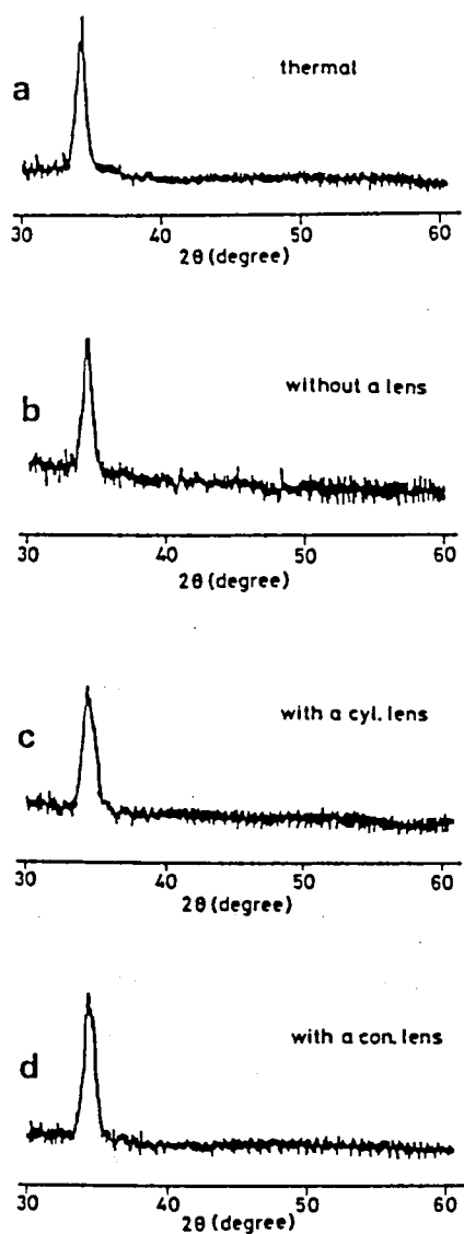
Fig.7.9. X-ray diffraction patterns of ZnO films grown at 200^\circ\text{C} by: (a) MOCVD; (b) photo-MOCVD (without a lens); (c) photo-MOCVD (with a cylindrical lens); (d) photo-MOCVD (with a convex lens). In photo-MOCVD, laser beams passed above the substrates.
