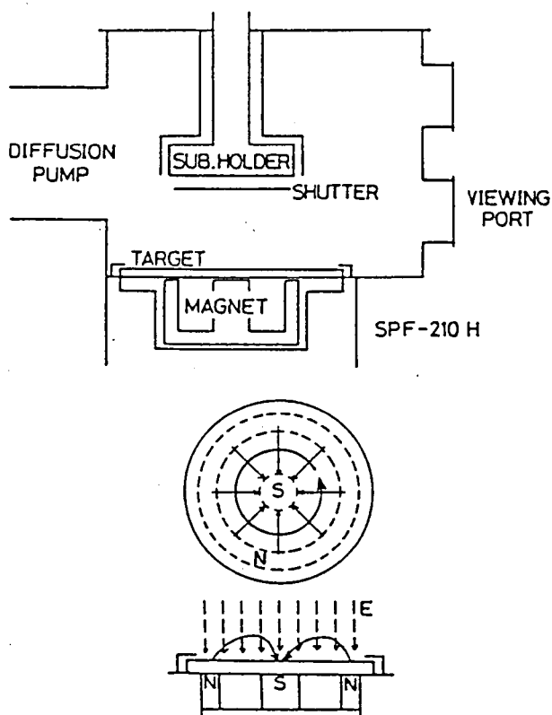
Fig.2.1. Sputtering chamber and magnetron cathode.
