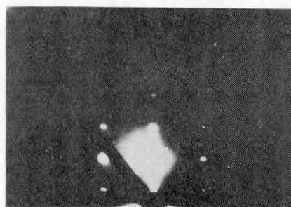
Fig.2.7. X-ray Laue back reflection pattern of (11\bar{2}0) ZnO and (01\bar{1}2) sapphire.
