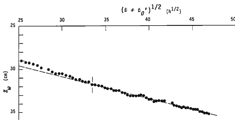
Fig. 21. Relation between z_w and (t+t_0')^{1/2} , corresponding to Fig. 20.
