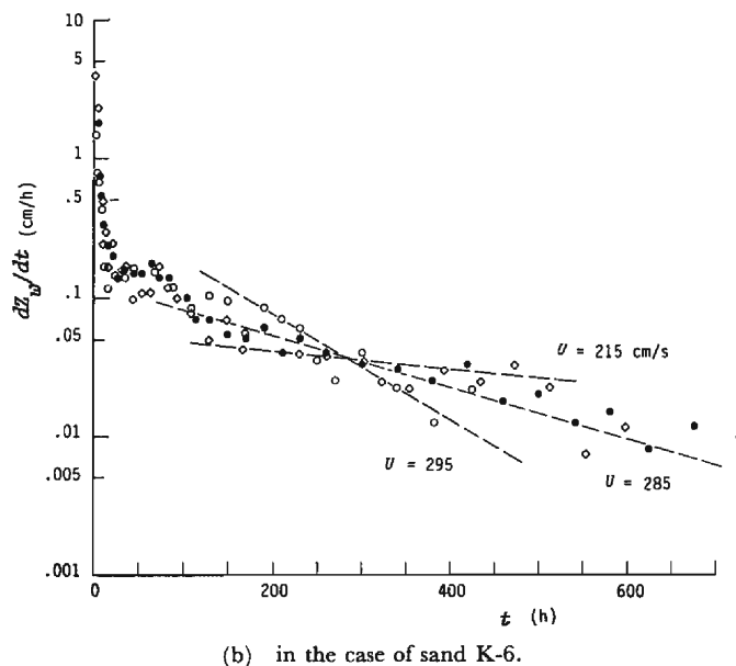
Fig. 24. Changes of dz_w/dt with time.
