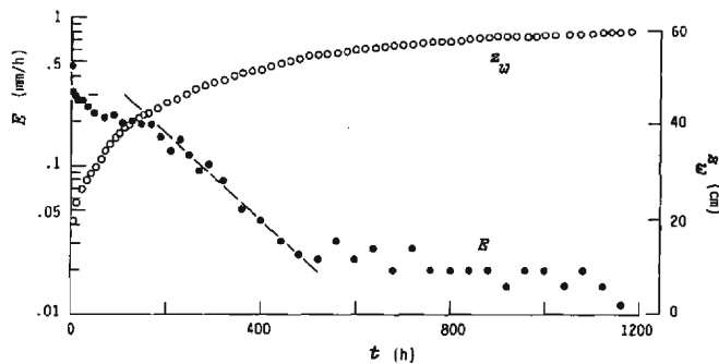
Fig. 7. Changes in the evaporation rate and the water table depth with time for Sand K-6 and U=285\text{ cm/s} .
