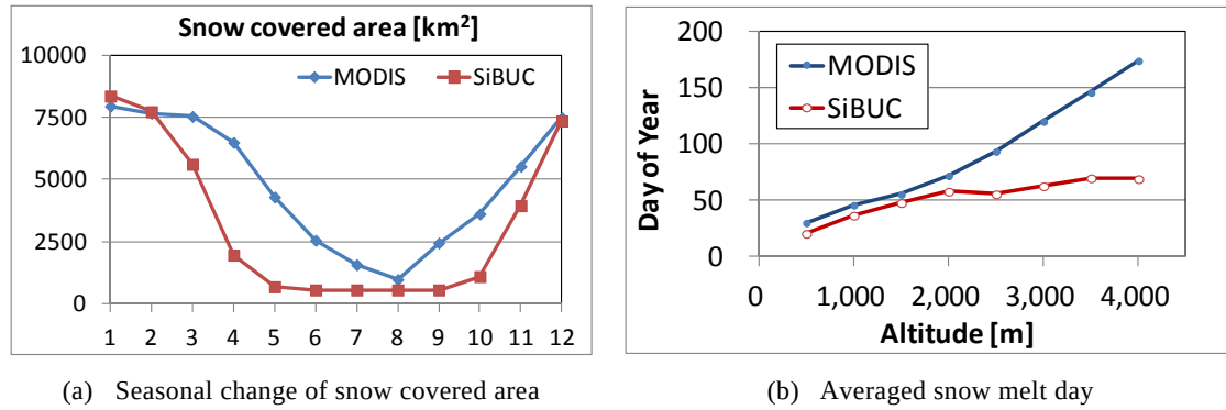
Fig.4 Comparison of snow area between analyzed result and satellite data
