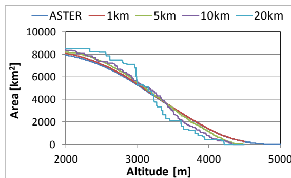
Fig.6 Area more than each altitude
