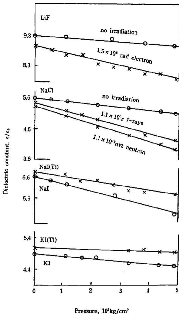
Fig. 10 The pressure dependance of the dielectric constants of alkali halide crystals irradiated by \gamma -ray, electron and neutron beams and activated by Thallous ions
