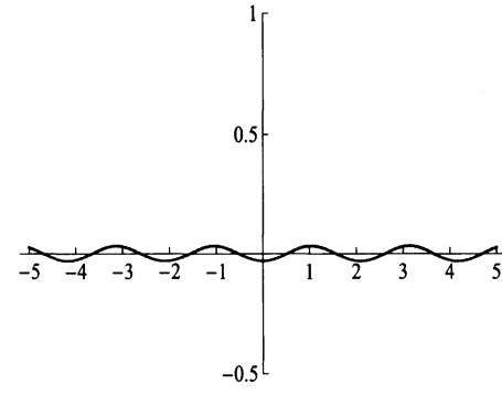
(f) \text{Im } \varphi_8^{ST}
