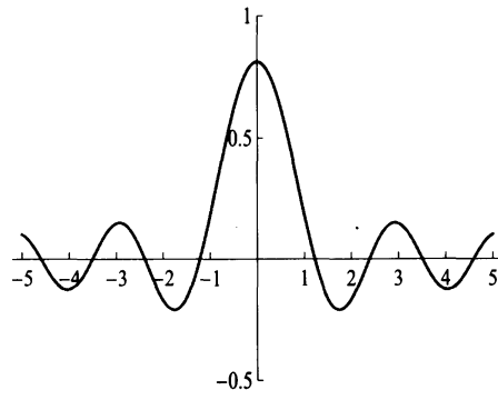
(c) \text{Re } \varphi_5^{ST}
