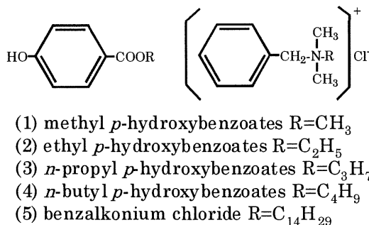
Fig.1-1 Structures of p -hydroxybenzoates (A) and benzalkonium chloride (B).
