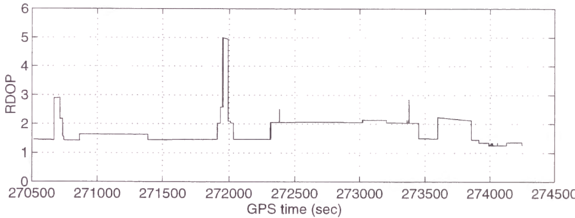
Fig.4-21 Variation of RDOP during the flight test
