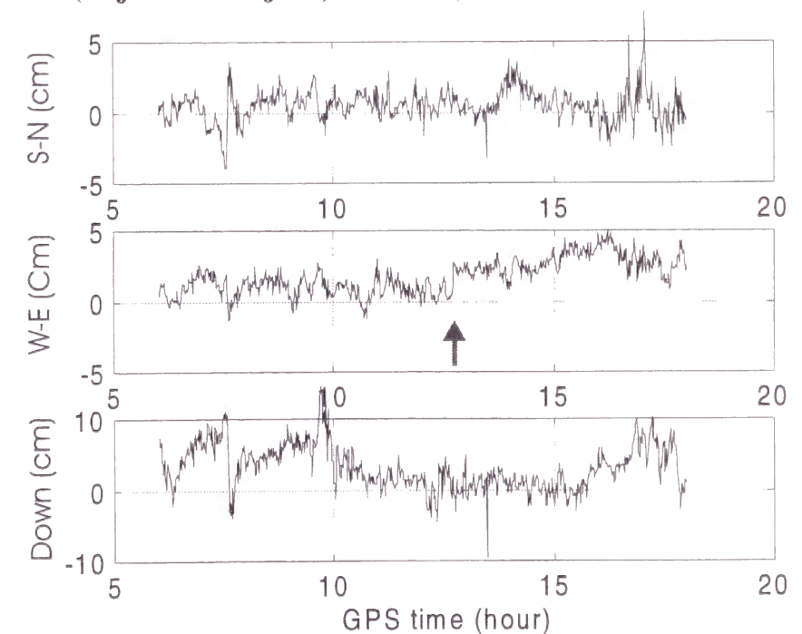
Fig.3-19a Position of Kozujima estimated by kinematic GPS before and after an earthquake that occurred at 12h43m, DOY279. (Nijijima - Kozujima, 22.146km)
