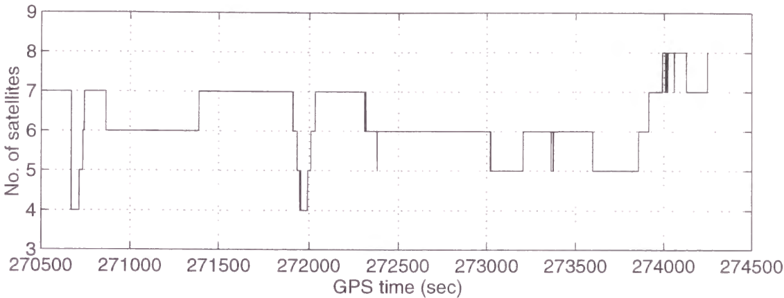
Fig.4-20 Number of satellites observed during the flight test
