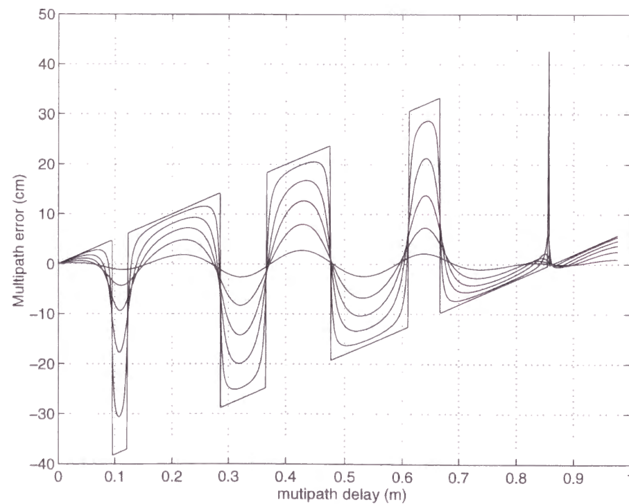
Fig.3-11a Multipath errors on widelane observable
