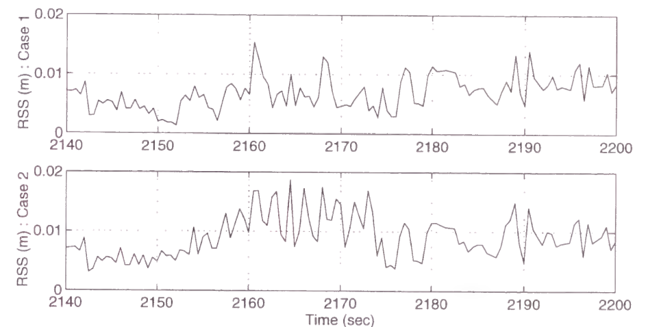
Fig.4-38 Root-Sum-Squares (RSS) of residuals in the estimation process for Case 1 (upper) and Case 2 (lower)
