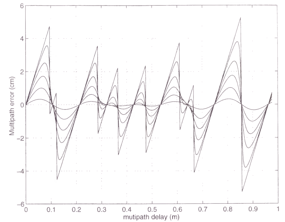
Fig.3-11b Multipath errors on narrowlane observable
