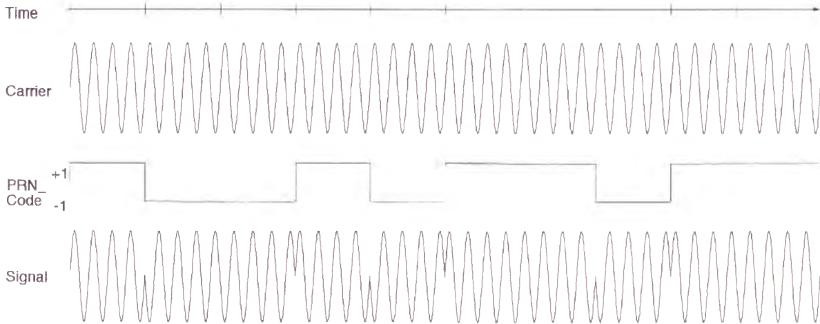
Fig.2-2 Structure of the GPS satellite signal
