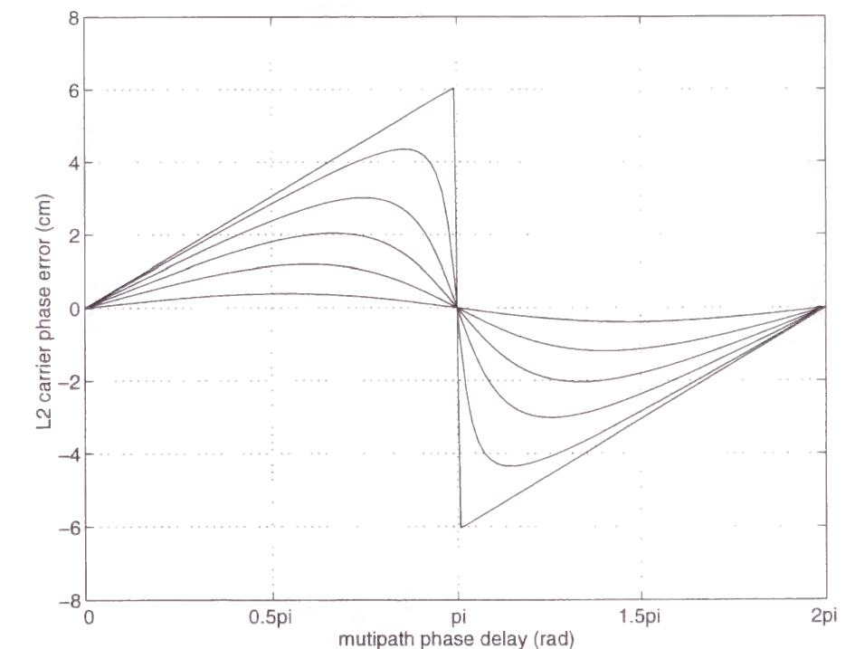
Fig.3-9b Multipath errors on L2 carrier phase for various damping factors
