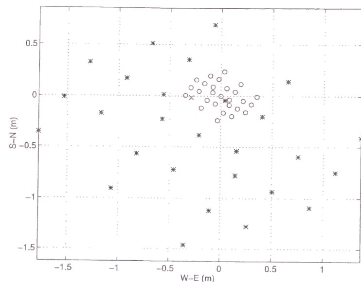
Fig.4-26 Horizontal position of the receiver using smoothed pseudorange (x), widelane ambiguity candidates (*), and L1 phase ambiguity candidates (o)
