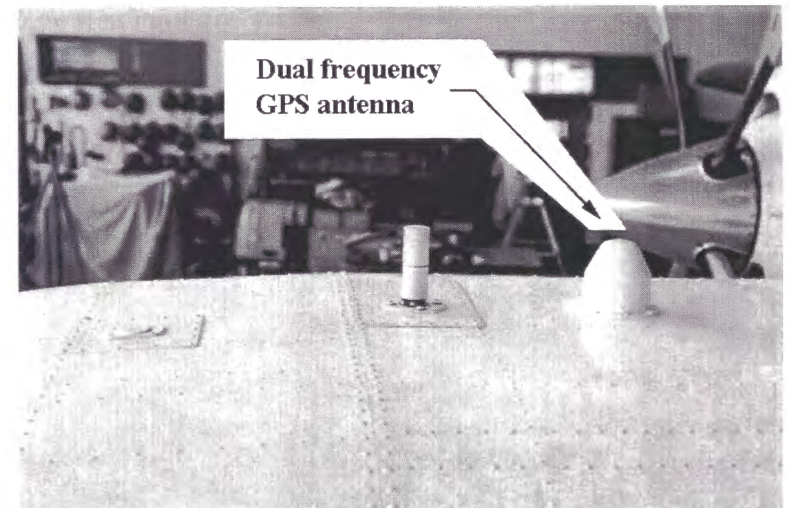
Fig.4-4 Dual frequency GPS antenna (Tecom MIL-E-5400) mounted on the roof of Do-228
