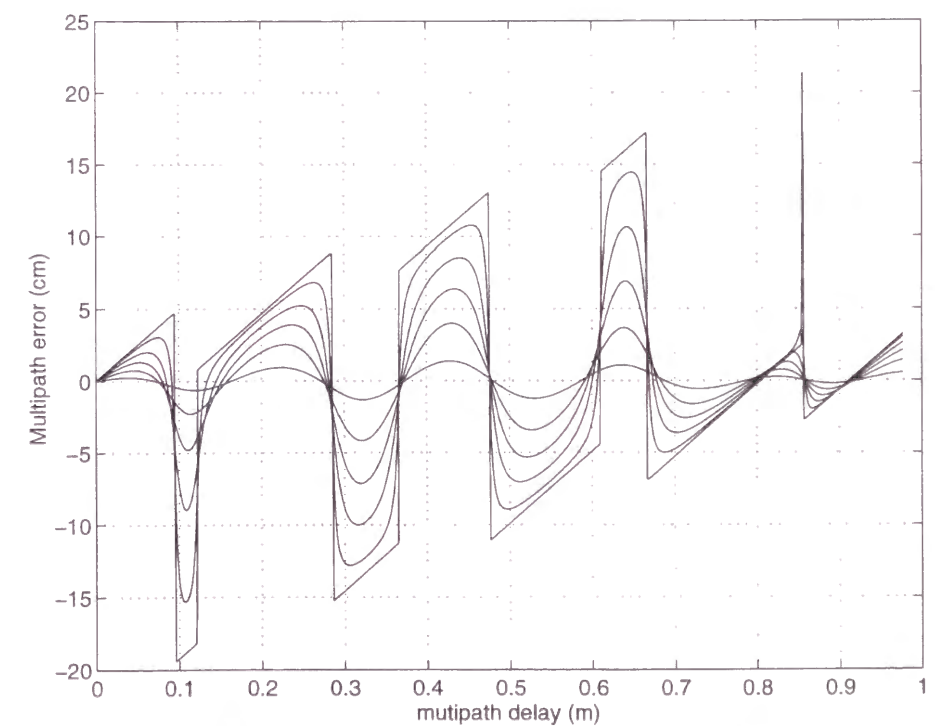
Fig.3-11c Multipath errors on ionospheric-free observable
