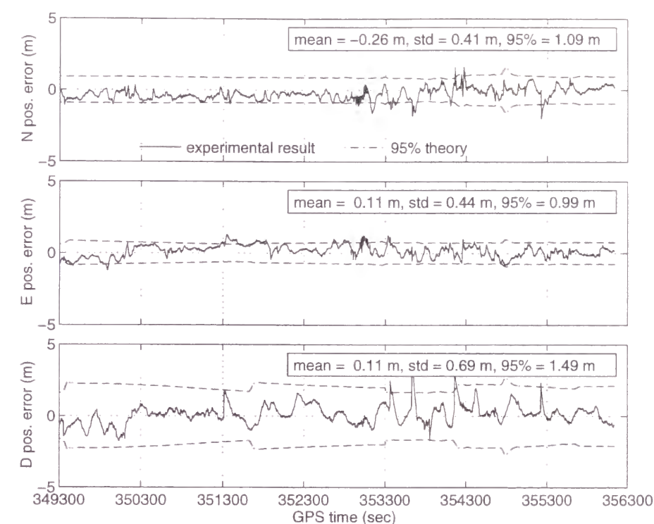
Fig.4-15 Position difference between the DGPS/INS and KGPS
