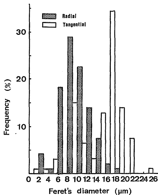
Fig. 9. Frequency of Feret's diameter of fibre lumen at the center of an annual ring of makanba.
