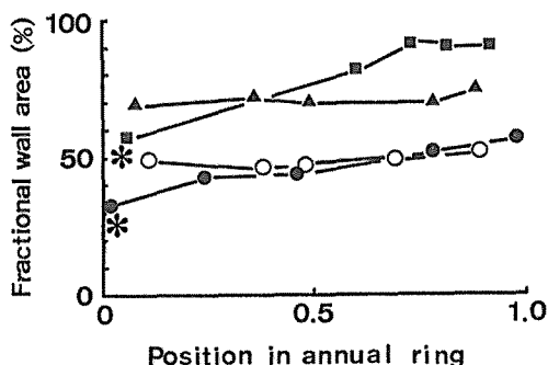
Fig. 8. Variation of fractional wall area of fibre within an annual ring.
