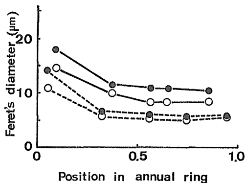
Fig. 3. Variation of Feret's diameter of fibre lumen within an annual ring in ring-porous wood (2).
