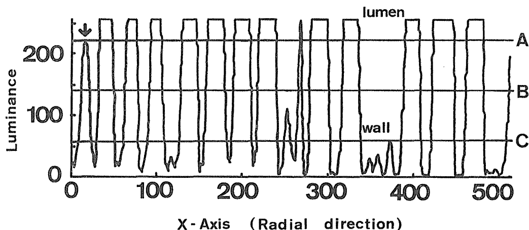
Fig. 1. Determination of threshold level on a profile of each sample section. Arrow indicates the luminance at the boundary between cell wall and lumen. Luminance: A < lumen, C > cell wall, B = threshold level (average value of A and C).
