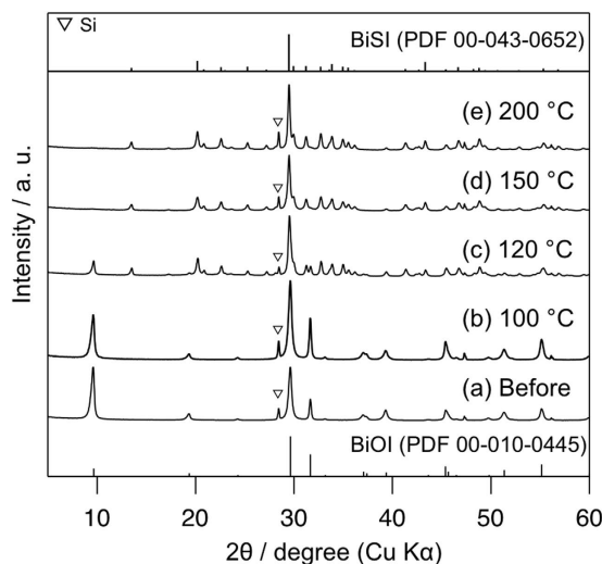
Figure 1. XRD patterns of the prepared samples (a) before and after heat treatment with 5% \text{H}_2\text{S} gas at (b) 100 °C, (c) 120 °C, (d) 150 °C, and (e) 200 °C.
