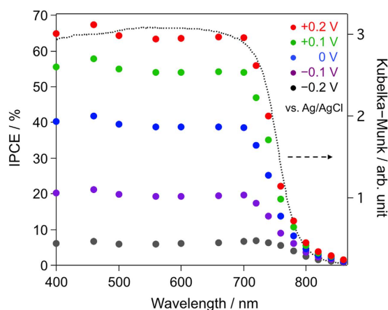
Figure 5. IPCE spectra of the BiSI electrode in an acetonitrile solution containing 0.1 M NaI at various applied potentials and absorption spectrum of BiSI.
