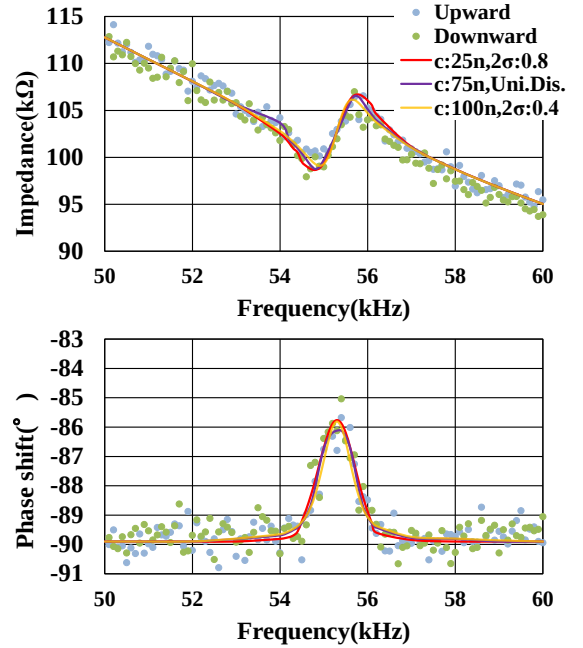
Figure 6: Impedance spectra at 100 Pa with 35 mVac and 0.5 Vdc bias. Fitting curves show assumed different estimated deviations of resonant frequencies.
