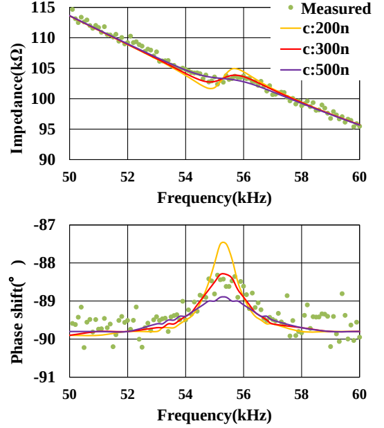
Figure 5: Impedance spectra at 1 kPa with 35 mVac and 0.5 Vdc bias. Fitting curves show different damping factors.
