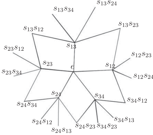
Figure 2: Neighborhood of e in the Cayley complex C_4^{[2,3]}
