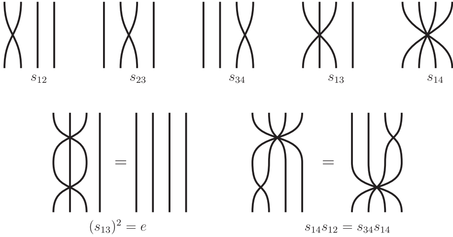
Figure 1: Diagrams for some elements of J_4
