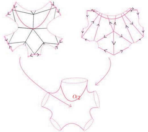
Figure 6: Finding the generator \alpha_2
