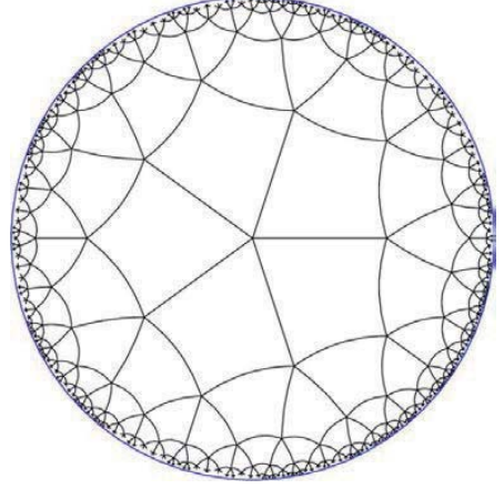
Figure 3: The \{4,5\} -tessellation of the hyperbolic plane. ([2, Figure 7])
