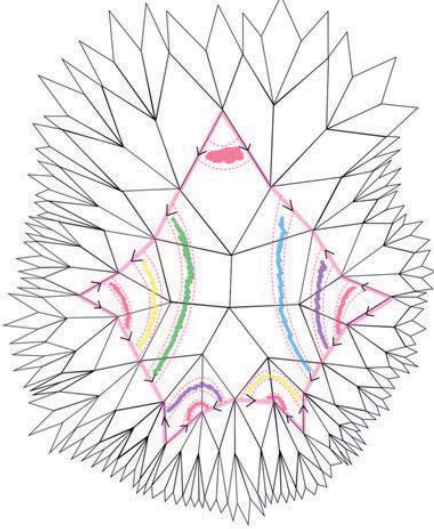
Figure 5: Five Möbius bands
