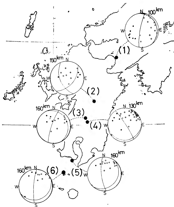
Fig. 7. Focal mechanism of the intermediate events.
