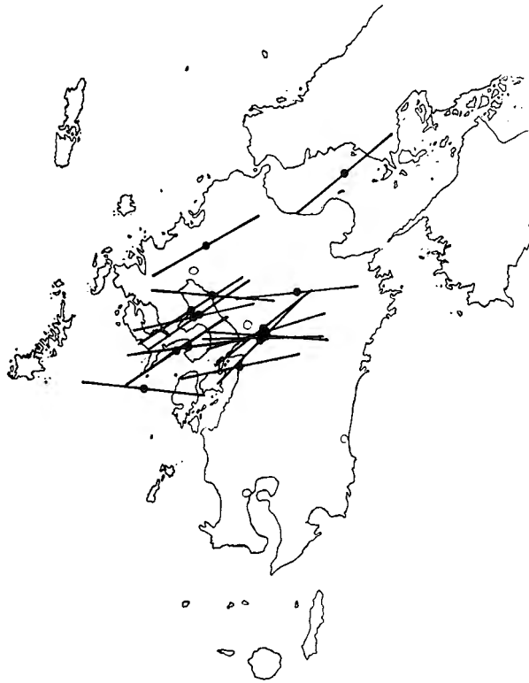
Fig. 6. Direction of the compression axes in the western area of Kyushu Island.
