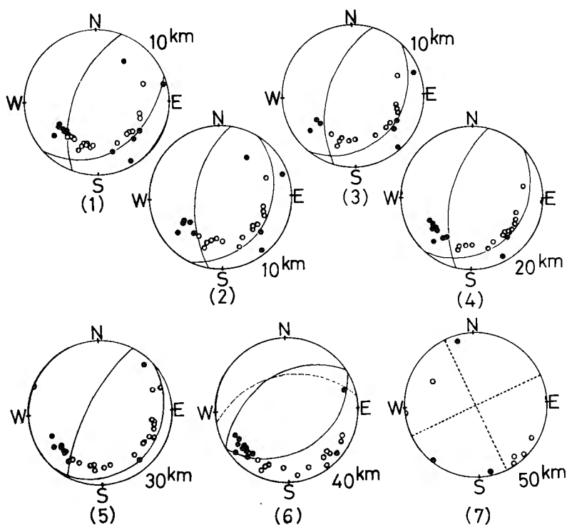
Fig. 4. Focal mechanism in the Hyuga Sea.
