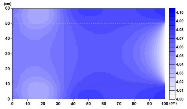
Fig. 5 Result of water level (2D model)
