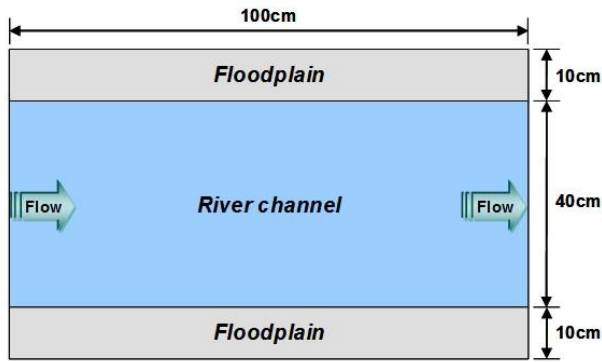
Fig. 2 Computational domain
