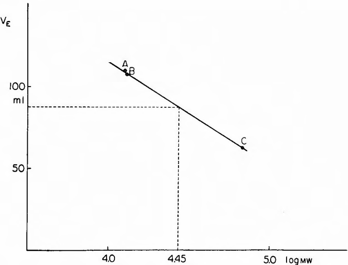
Fig. 12. Molecular weight of S-100 protein was assayed on Sephadex G-100 column chromatography. A, RNase A ; B, Cytochrome C ; C, Crystalline bovine albumin.
