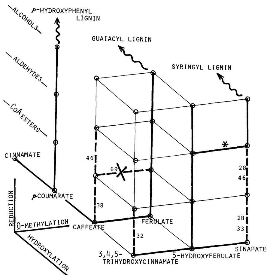
Figure 18 Possible biosynthetic pathways in the formation of syringyl lignin. \bigcirc — \bigcirc convertible reactions in vitro , \bigcirc — \bigcirc low reaction rate or no reaction in vitro , \bigcirc — \bigcirc possible pathway for syringyl lignin biosynthesis. Numbers in this figure indicate reference numbers. * Kutsuki et al. unpublished result.
