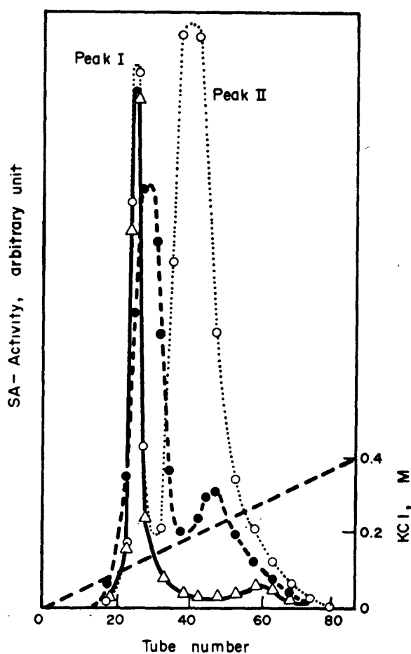
Figure 7 Elution profiles of aspen OMTs from DEAE-cellulose column chromatography. ...○... A crude juice corresponding to step 1, --●-- step 3 in the Table 7, —△— re-chromatogram after step 3 (kept in a refrigerator more than 2 weeks)
