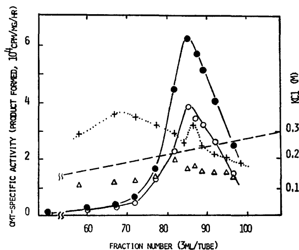
Figure 9 Elution pattern of bamboo OMT on a DEAE-cellulose column. —○— FA-activity, —●— SA-activity, \Delta SA/FA ratio, ...+... protein concentration
