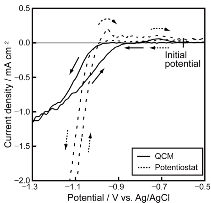
Figure 3.6 Cyclic voltammograms measured at 1 \text{ mV s}^{-1} in EG containing containing 0.050 \text{ M} \text{CoCl}_2 \cdot 6\text{H}_2\text{O} and 1.0 \text{ M} \text{NaOH} by a potentiostat (dotted line) and QCM (solid line). The initial potential is -0.64 \text{ V} .
