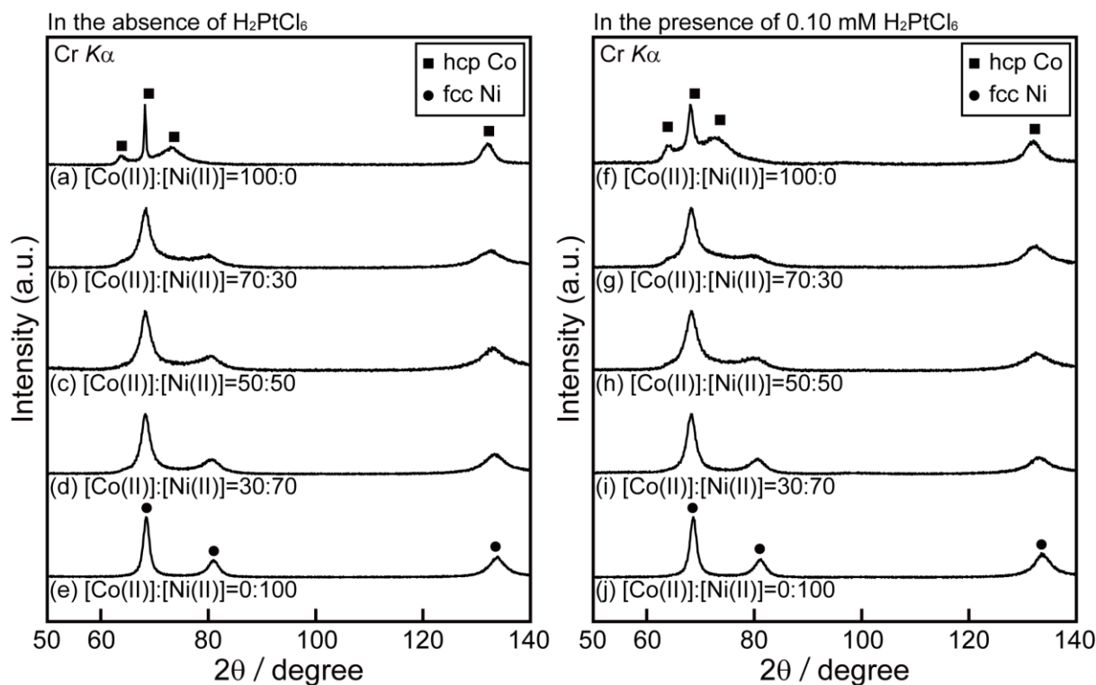
Figure 5.3 XRD patterns of the particles synthesized from the solutions containing (a) 0.050 M Co(II), (b) 0.035 M Co(II) - 0.015 M Ni(II), (c) 0.025 M Co(II) - 0.025 M Ni(II), (d) 0.015 M Co(II) - 0.035 M Ni(II), (e) 0.050 M Ni(II) in the absence of \text{H}_2\text{PtCl}_6 , and (f) 0.050 M Co(II), (g) 0.035 M Co(II) - 0.015 M Ni(II), (h) 0.025 M Co(II) - 0.025 M Ni(II), (i) 0.015 M Co(II) - 0.035 M Ni(II), (j) 0.050 M Ni(II) in the presence of 0.10 mM \text{H}_2\text{PtCl}_6 .
