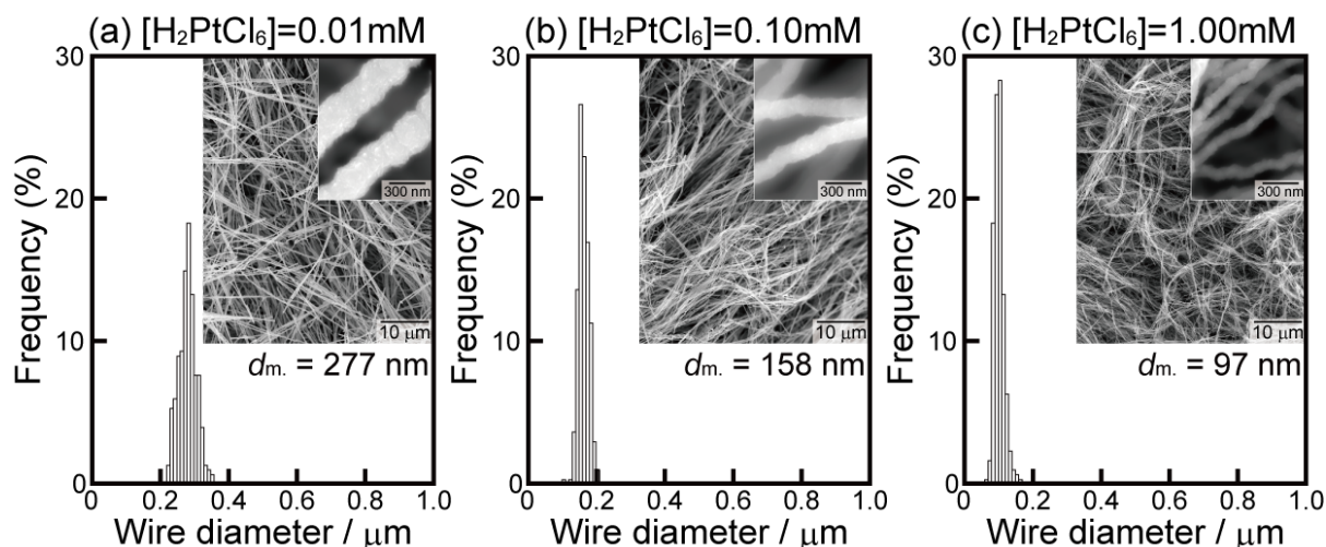
Figure 4.11 SEM images and size distribution of nickel wires synthesized from solutions containing 0.050 M \text{NiCl}_2 , 0.50 M \text{N}_2\text{H}_4 , 1.0 M \text{NaOH} , 10.0 mM \text{Na}_3\text{C}_6\text{H}_5\text{O}_7 , (a) 0.01 mM, (b) 0.10 mM, and (c) 1.00 mM \text{H}_2\text{PtCl}_6 . Mean diameter d_m is also indicated.
