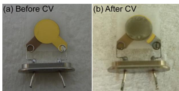
Figure 3.7 Photos of the QCM substrates (a) before and (b) after the CV measured at 1 \text{ mV s}^{-1} in 120 \text{ cm}^3 of EG containing 0.050 \text{ M} \text{CoCl}_2 \cdot 6\text{H}_2\text{O} and 1.0 \text{ M} \text{NaOH} .
