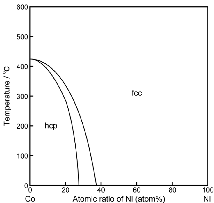
Figure 5.4 Phase diagram of the Co-Ni binary system. 8
