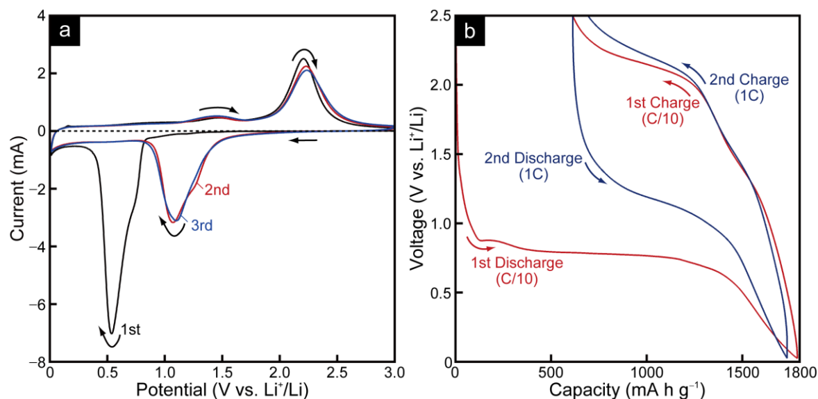
Figure 7.6 (a) Cyclic voltammogram of the NNNC annealed at 523 K measured at a scan rate of 0.1 mV s -1 in a solution of 33% ethylene carbonate and 67% dimethyl carbonate containing 1 M LiPF 6 . The cycle numbers are indicated in the graph. (b) Galvanostatic charge-discharge curves of the NNNC annealed at 523 K in the voltage range 0.02–2.50 V (vs. Li + /Li) at a rate of C/10 and 1 C for the first and second cycles, respectively.
