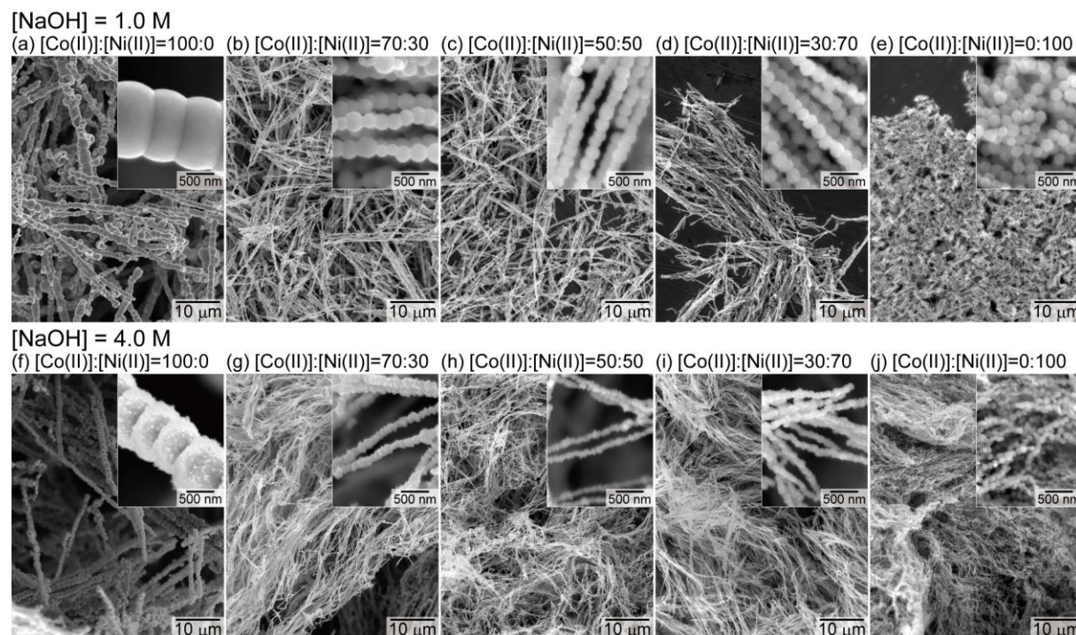
Figure 5.15 SEM images of the wires synthesized from the solutions containing (a) 0.050 M Co(II), (b) 0.035 M Co(II) - 0.015 M Ni(II), (c) 0.025 M Co(II) - 0.025 M Ni(II), (d) 0.015 M Co(II) - 0.035 M Ni(II), and (e) 0.050 M Ni(II) at 1.0 M NaOH, and (f) 0.050 M Co(II), (g) 0.035 M Co(II) - 0.015 M Ni(II), (h) 0.025 M Co(II) - 0.025 M Ni(II), (i) 0.015 M Co(II) - 0.035 M Ni(II), and (j) 0.050 M Ni(II) at 4.0 M NaOH.
