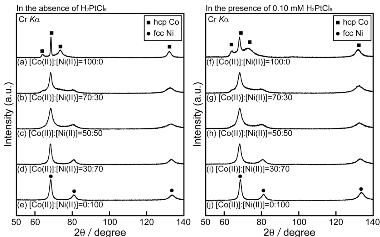
Figure 5.9 XRD patterns of the wires synthesized from the solutions containing (a) 0.050 M Co(II), (b) 0.035 M Co(II) - 0.015 M Ni(II), (c) 0.025 M Co(II) - 0.025 M Ni(II), (d) 0.015 M Co(II) - 0.035 M Ni(II), and (e) 0.050 M Ni(II) in the absence H 2 PtCl 6 , and (f) 0.050 M Co(II), (g) 0.035 M Co(II) - 0.015 M Ni(II), (h) 0.025 M Co(II) - 0.025 M Ni(II), (i) 0.015 M Co(II) - 0.035 M Ni(II), and (j) 0.050 M Ni(II) in the presence of 0.10 mM H 2 PtCl 6 .
