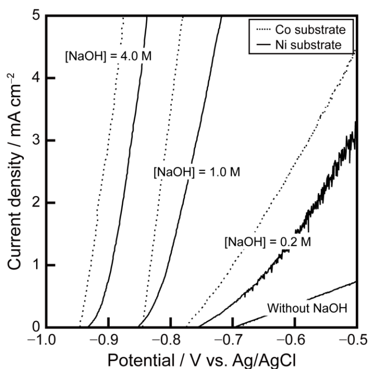
Figure 5.17 Anodic polarization curves measured on cobalt and nickel substrates in EG containing 0.50 M N 2 H 4 at various concentrations of NaOH. Sweep rate is 1 mV s -1 . The supporting electrolyte, 0.1 M LiClO 4 , was added in the solutions without NaOH. During the measurement, the temperature of the solutions was kept at a reaction temperature of 353 K on a hot plate with nitrogen gas bubbling to remove the dissolved oxygen.
