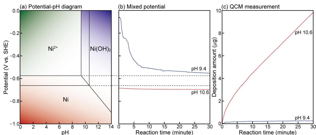
Figure 7.1 (a) Potential–pH diagrams drawn at the equilibrium activities of \text{Ni}^{2+} aquo ions at pH 9.4 and 10.6 at 353 K considering the chemical species of \text{Ni}^{2+} , \text{Ni(OH)}_2 , \text{Ni} , \text{H}_2\text{O} , \text{H}^+ , and \text{OH}^- . (b) Time dependence of mixed potential and (c) weight change of metal deposited on the gold-sputtered QCM substrate immersed in the solution containing 0.050 M \text{Ni(II)} and 0.50 \text{N}_2\text{H}_4 at pH 9.4 and 10.6.
