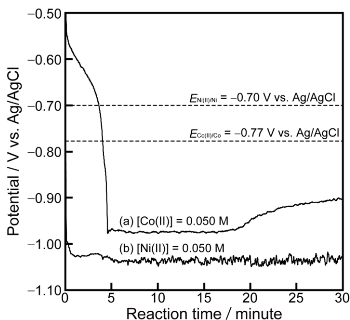
Figure 5.12 Time dependence of mixed potential in the solution containing 0.50 \text{N}_2\text{H}_4 , 0.2 M NaOH, and (a) 0.050 M Co(II) or (b) 0.050 M Ni(II).
