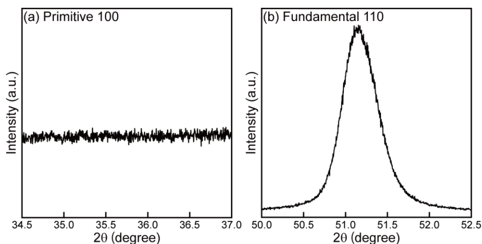
Figure 6.4 Synchrotron XRD patterns of the Fe 42 Co 58 particles synthesized from the solutions containing 0.070 M Co(II) - 0.030 M Fe(II) for selected regions; (a) primitive 100 and (b) fundamental 110 reflections. The X-ray wavelength was chosen to be 1.7434 Å near the Fe K edge.
