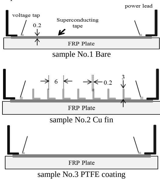
Fig. 1. Schema of test superconducting tapes for all samples
