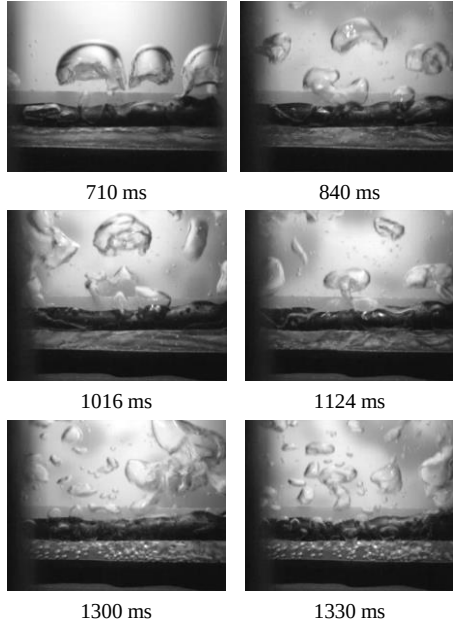
Fig. 8. Boiling behavior during quench and recovery for sample No.3.
