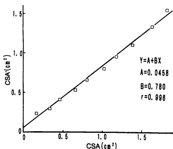
Fig. 2. Correlation between CSA' and CSA . CSA' : cross sectional area measured by caliper ( \text{cm}^2 ), CSA : cross sectional area measured by balloon probe ( \text{cm}^2 ).
